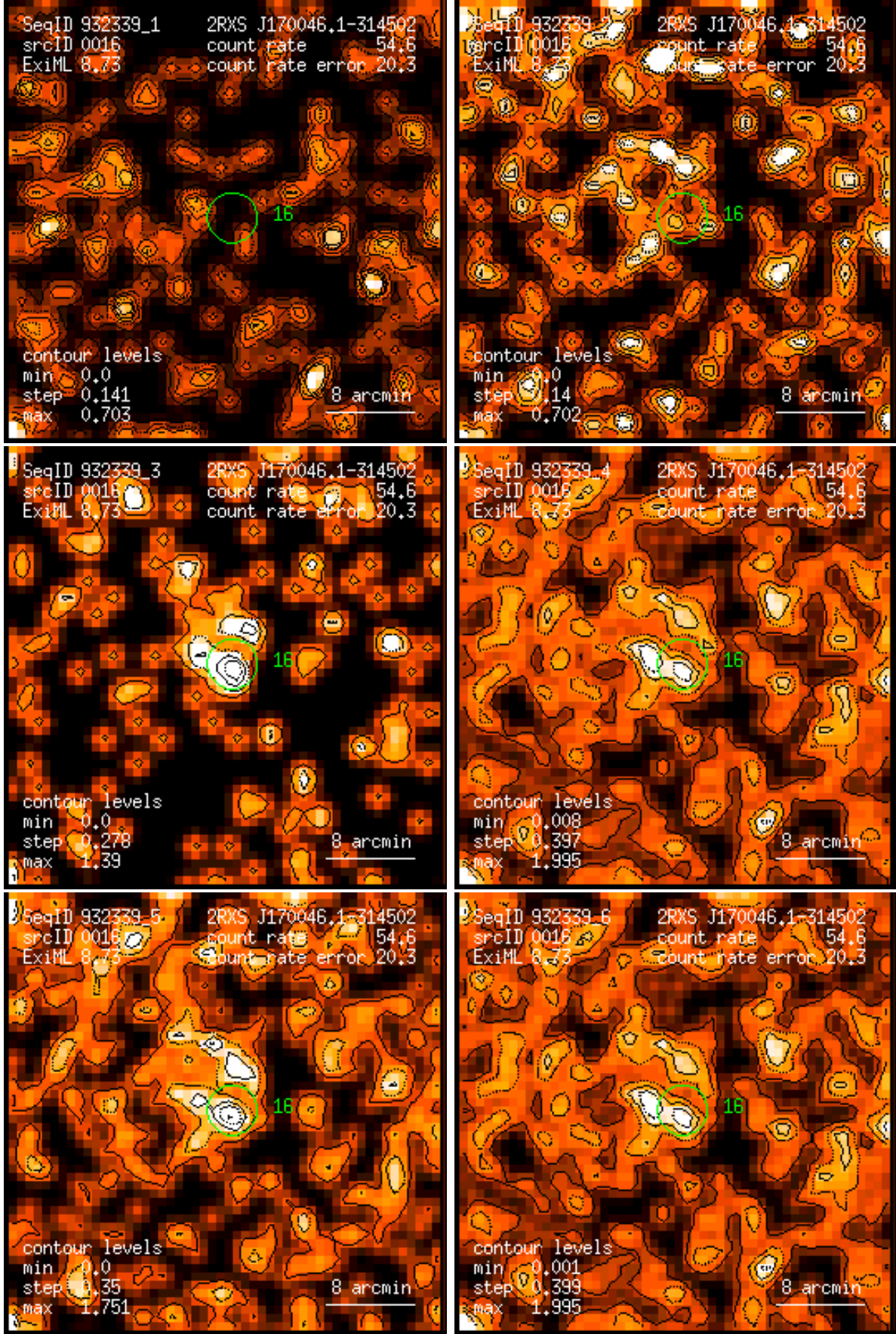
Figure 16: RASS 932339: detection 0016: band rate images, Gaussian filter: (1) PSPC channels 11 – 41, (2) 52 – 90, (3) 91 – 201, (4) 11 – 235, (5) 52 – 201, (6) 11 – 201. Broad band rates in counts/ks. Band rate contour levels in counts/ks/arcmin 2 .
