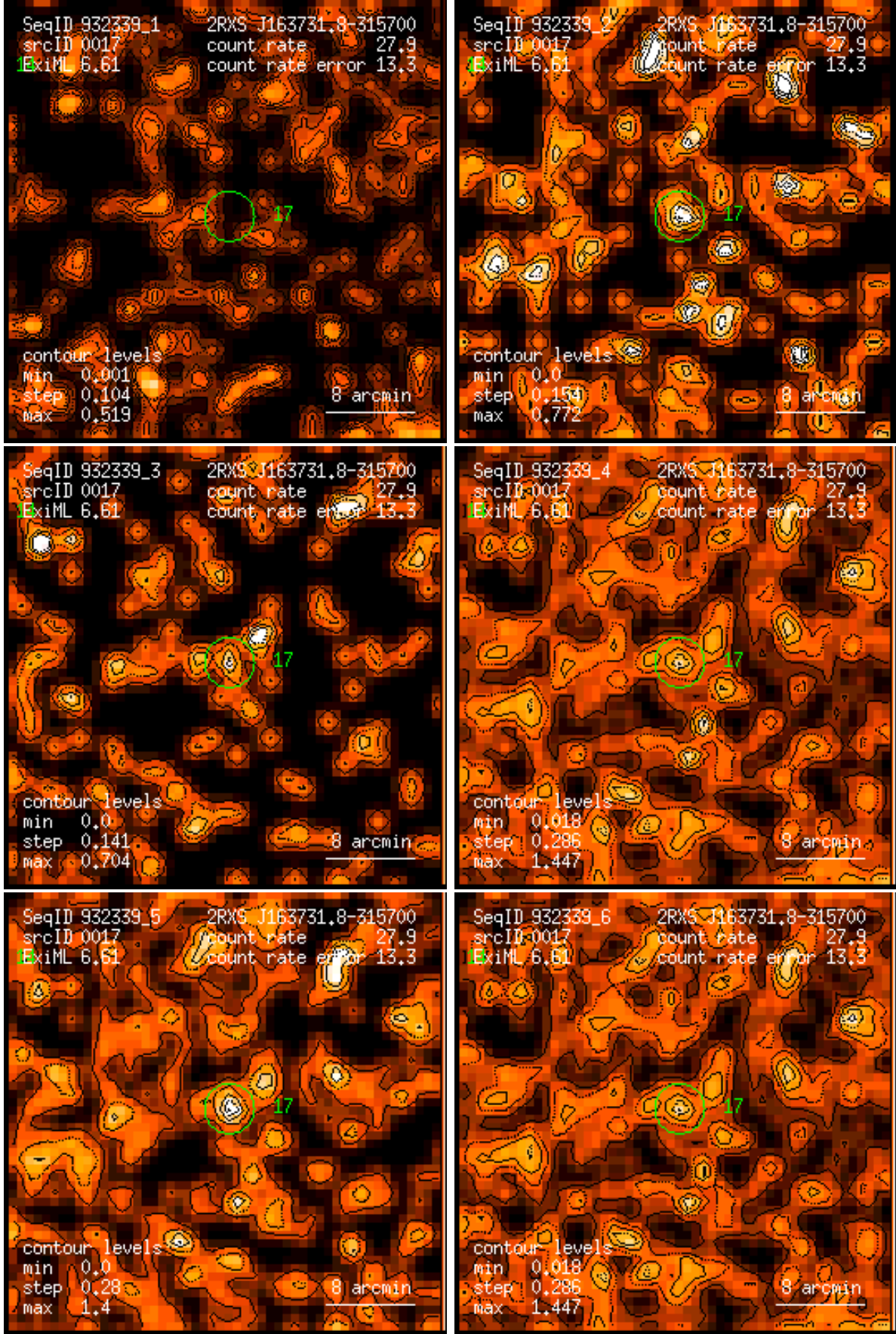
Figure 17: RASS 932339: detection 0017: band rate images, Gaussian filter: (1) PSPC channels 11 – 41, (2) 52 – 90, (3) 91 – 201, (4) 11 – 235, (5) 52 – 201, (6) 11 – 201. Broad band rates in counts/ks. Band rate contour levels in counts/ks/arcmin 2 .
