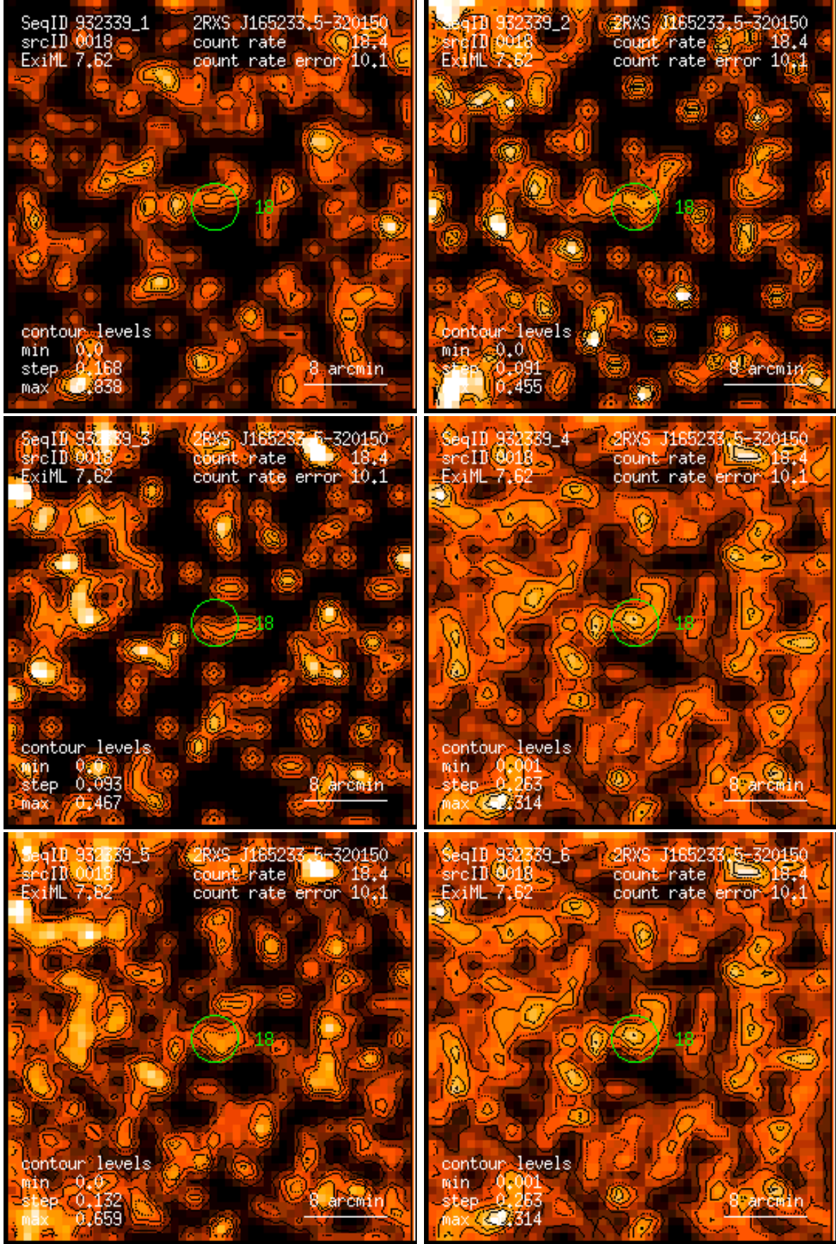
Figure 18: RASS 932339: detection 0018: band rate images, Gaussian filter: (1) PSPC channels 11 – 41, (2) 52 – 90, (3) 91 – 201, (4) 11 – 235, (5) 52 – 201, (6) 11 – 201. Broad band rates in counts/ks. Band rate contour levels in counts/ks/arcmin 2 .
