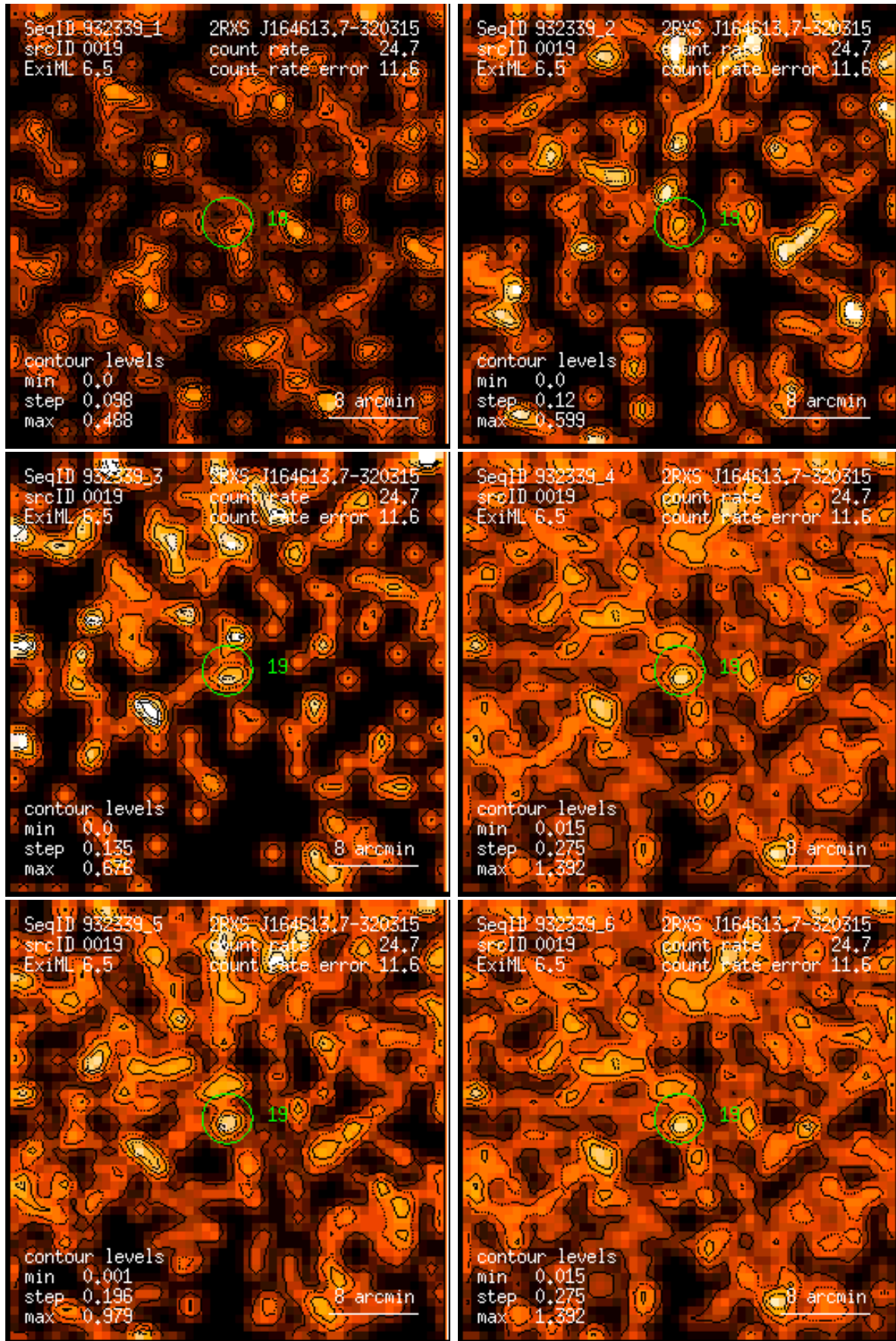
Figure 19: RASS 932339: detection 0019: band rate images, Gaussian filter: (1) PSPC channels 11 – 41, (2) 52 – 90, (3) 91 – 201, (4) 11 – 235, (5) 52 – 201, (6) 11 – 201. Broad band rates in counts/ks. Band rate contour levels in counts/ks/arcmin 2 .
