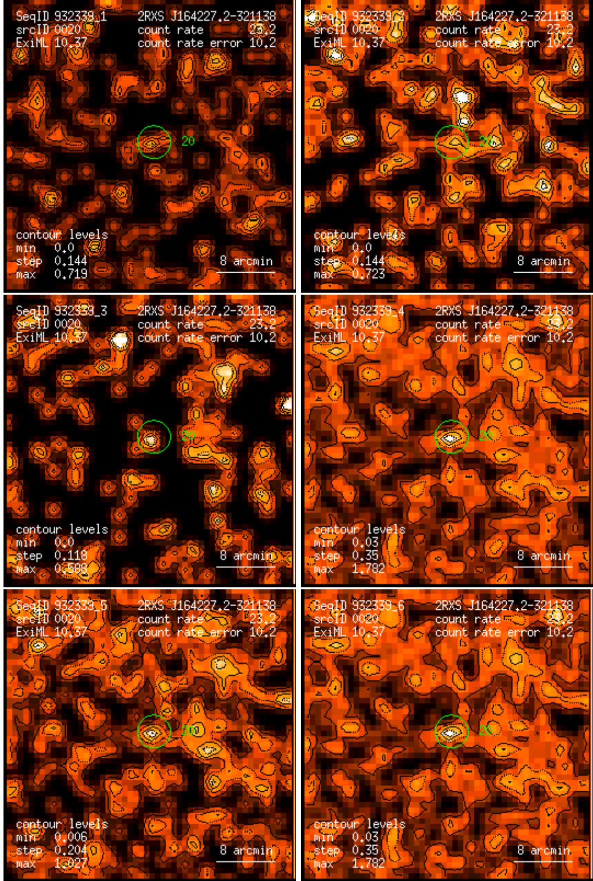
Figure 20: RASS 932339: detection 0020: band rate images, Gaussian filter: (1) PSPC channels 11 – 41, (2) 52 – 90, (3) 91 – 201, (4) 11 – 235, (5) 52 – 201, (6) 11 – 201. Broad band rates in counts/ks. Band rate contour levels in counts/ks/arcmin 2 .
