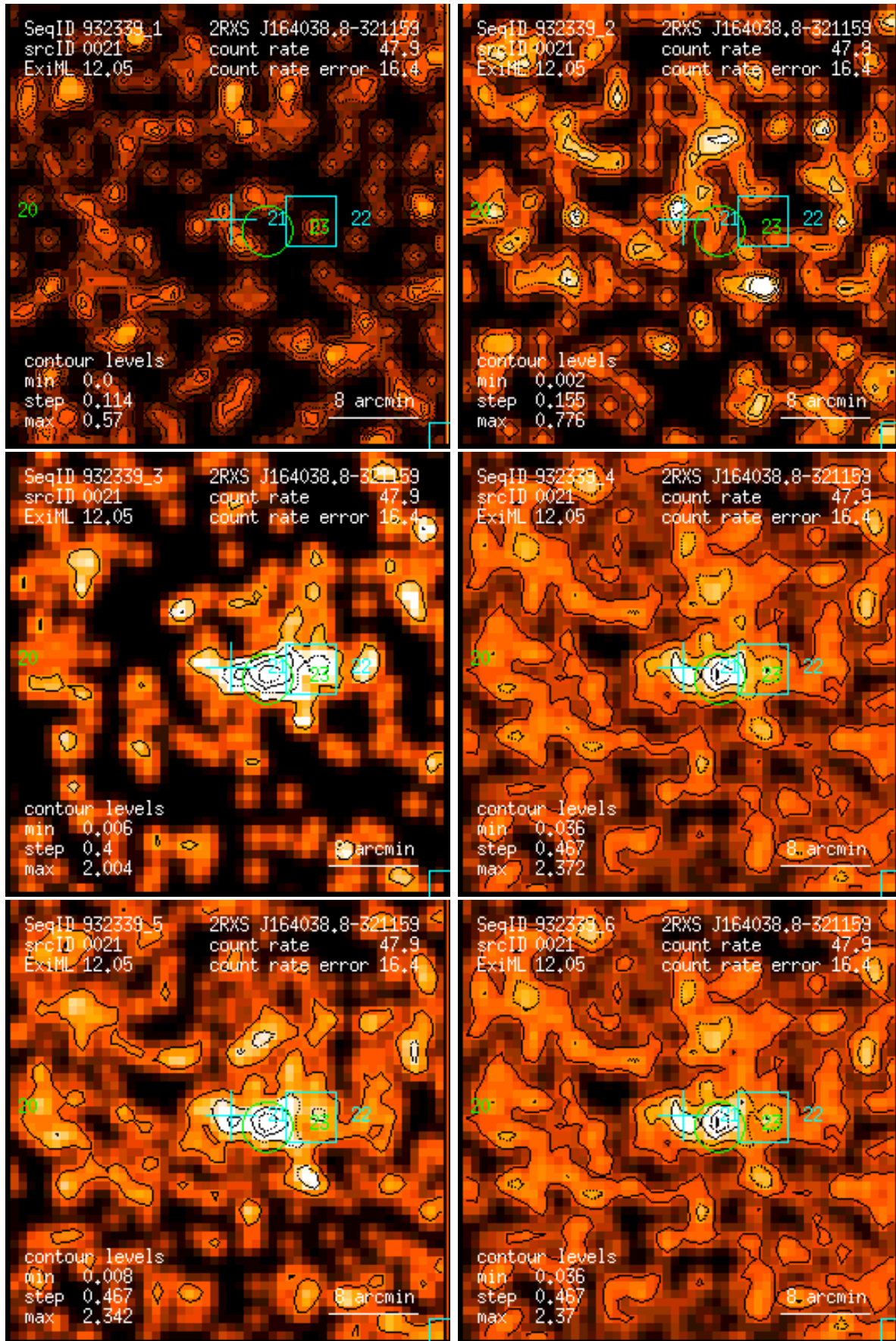
Figure 21: RASS 932339: detection 0021: band rate images, Gaussian filter: (1) PSPC channels 11 – 41, (2) 52 – 90, (3) 91 – 201, (4) 11 – 235, (5) 52 – 201, (6) 11 – 201. Broad band rates in counts/ks. Band rate contour levels in counts/ks/arcmin 2 .
