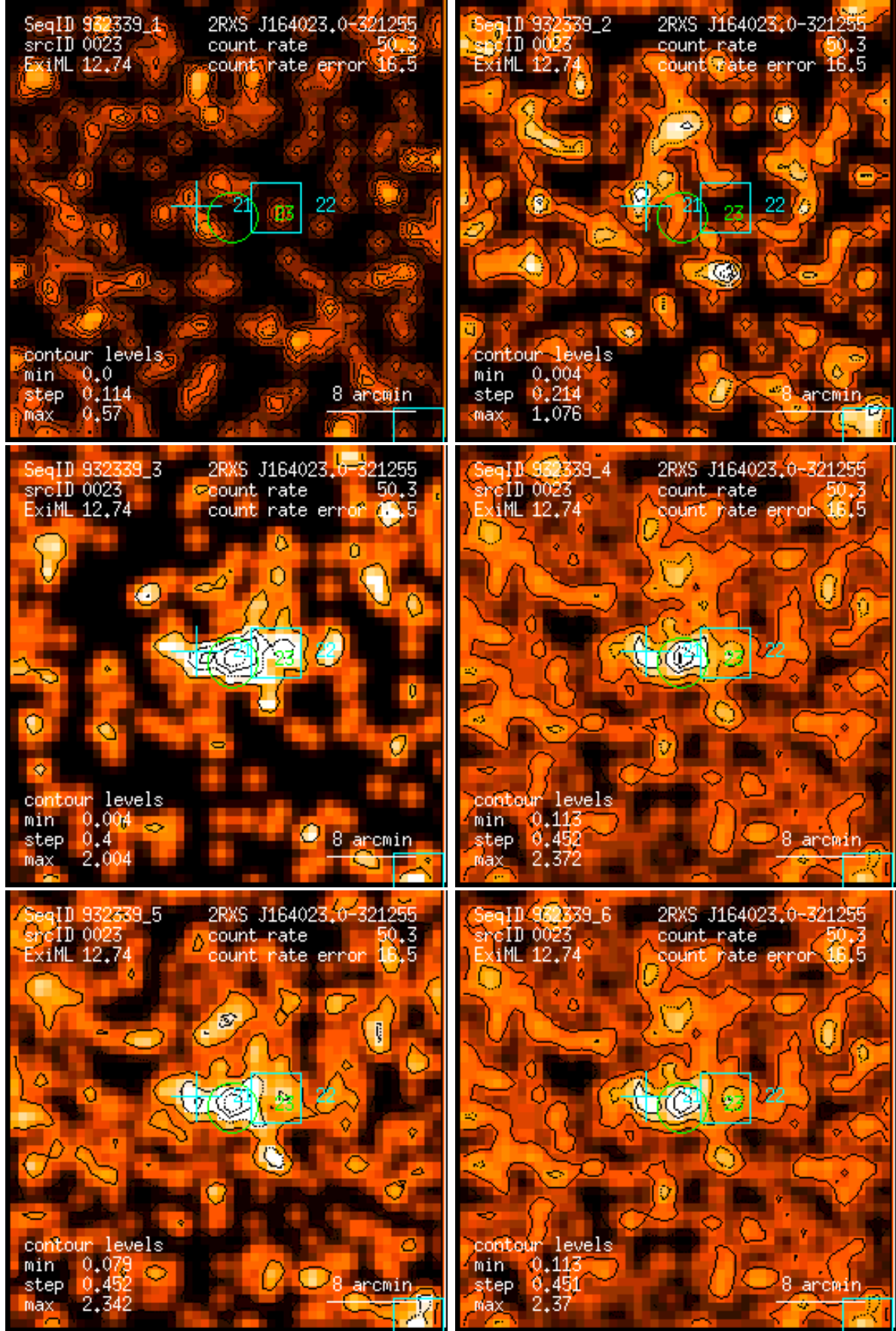
Figure 23: RASS 932339: detection 0023: band rate images, Gaussian filter: (1) PSPC channels 11 – 41, (2) 52 – 90, (3) 91 – 201, (4) 11 – 235, (5) 52 – 201, (6) 11 – 201. Broad band rates in counts/ks. Band rate contour levels in counts/ks/arcmin 2 .
