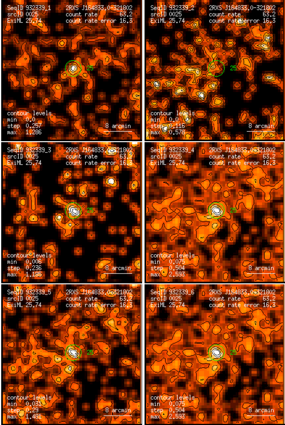
Figure 25: RASS 932339: detection 0025: band rate images, Gaussian filter: (1) PSPC channels 11 – 41, (2) 52 – 90, (3) 91 – 201, (4) 11 – 235, (5) 52 – 201, (6) 11 – 201. Broad band rates in counts/ks. Band rate contour levels in counts/ks/arcmin 2 .
