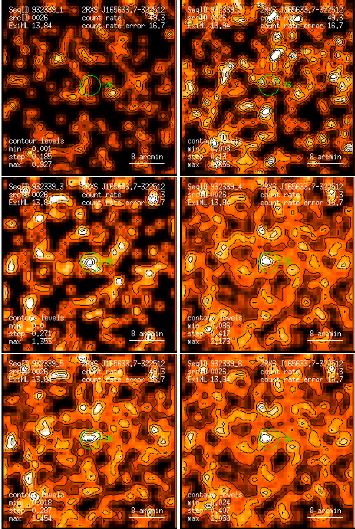
Figure 26: RASS 932339: detection 0026: band rate images, Gaussian filter: (1) PSPC channels 11 – 41, (2) 52 – 90, (3) 91 – 201, (4) 11 – 235, (5) 52 – 201, (6) 11 – 201. Broad band rates in counts/ks. Band rate contour levels in counts/ks/arcmin 2 .
