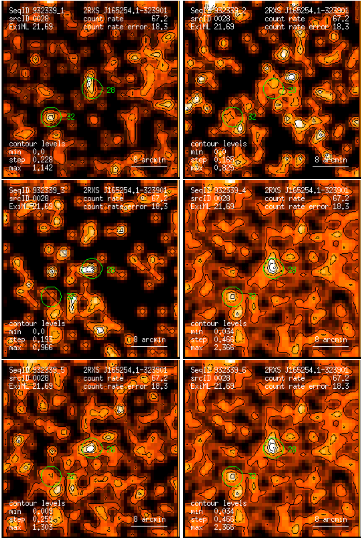
Figure 28: RASS 932339: detection 0028: band rate images, Gaussian filter: (1) PSPC channels 11 – 41, (2) 52 – 90, (3) 91 – 201, (4) 11 – 235, (5) 52 – 201, (6) 11 – 201. Broad band rates in counts/ks. Band rate contour levels in counts/ks/arcmin 2 .
