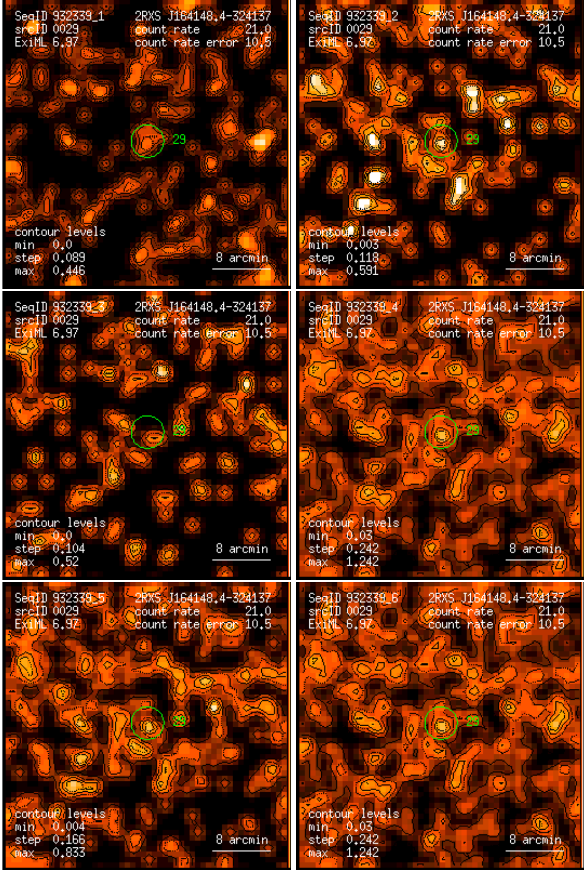
Figure 29: RASS 932339: detection 0029: band rate images, Gaussian filter: (1) PSPC channels 11 – 41, (2) 52 – 90, (3) 91 – 201, (4) 11 – 235, (5) 52 – 201, (6) 11 – 201. Broad band rates in counts/ks. Band rate contour levels in counts/ks/arcmin 2 .
