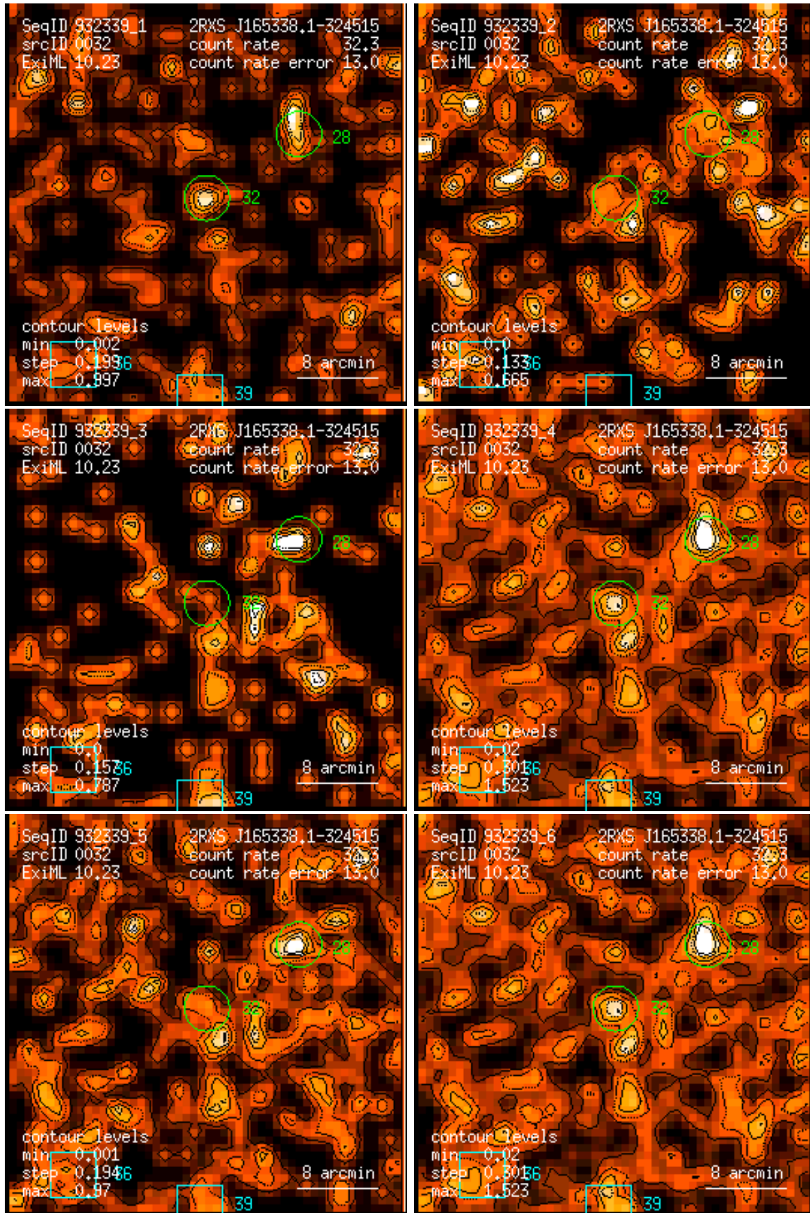
Figure 32: RASS 932339: detection 0032: band rate images, Gaussian filter: (1) PSPC channels 11 – 41, (2) 52 – 90, (3) 91 – 201, (4) 11 – 235, (5) 52 – 201, (6) 11 – 201. Broad band rates in counts/ks. Band rate contour levels in counts/ks/arcmin 2 .
