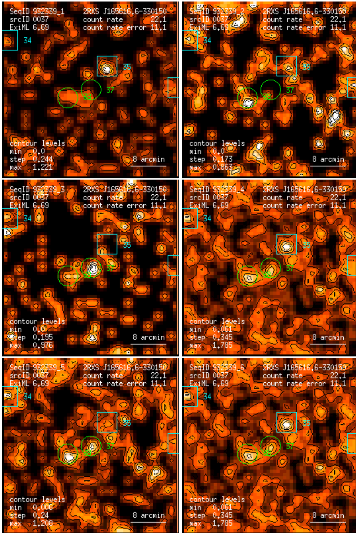
Figure 37: RASS 932339: detection 0037: band rate images, Gaussian filter: (1) PSPC channels 11 – 41, (2) 52 – 90, (3) 91 – 201, (4) 11 – 235, (5) 52 – 201, (6) 11 – 201. Broad band rates in counts/ks. Band rate contour levels in counts/ks/arcmin 2 .
