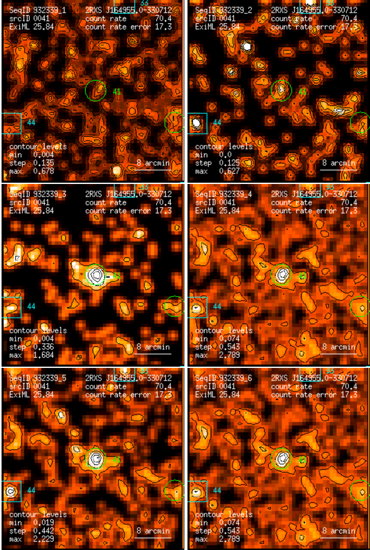
Figure 41: RASS 932339: detection 0041: band rate images, Gaussian filter: (1) PSPC channels 11 – 41, (2) 52 – 90, (3) 91 – 201, (4) 11 – 235, (5) 52 – 201, (6) 11 – 201. Broad band rates in counts/ks. Band rate contour levels in counts/ks/arcmin 2 .
