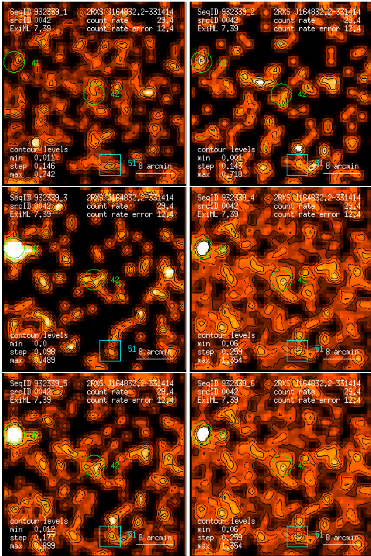
Figure 42: RASS 932339: detection 0042: band rate images, Gaussian filter: (1) PSPC channels 11 – 41, (2) 52 – 90, (3) 91 – 201, (4) 11 – 235, (5) 52 – 201, (6) 11 – 201. Broad band rates in counts/ks. Band rate contour levels in counts/ks/arcmin 2 .
