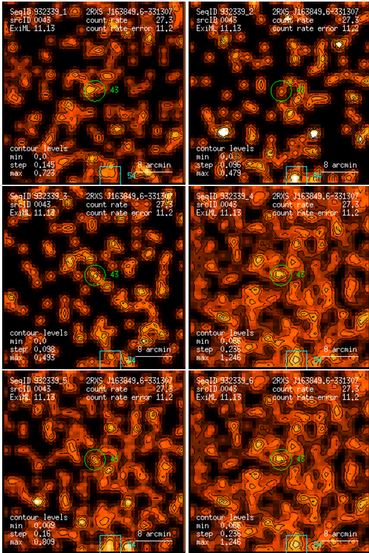
Figure 43: RASS 932339: detection 0043: band rate images, Gaussian filter: (1) PSPC channels 11 – 41, (2) 52 – 90, (3) 91 – 201, (4) 11 – 235, (5) 52 – 201, (6) 11 – 201. Broad band rates in counts/ks. Band rate contour levels in counts/ks/arcmin 2 .
