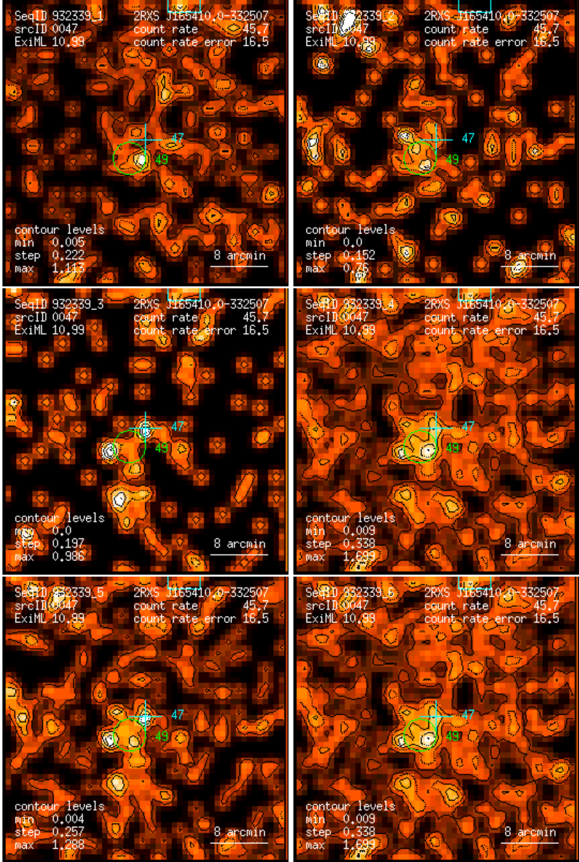
Figure 47: RASS 932339: detection 0047: band rate images, Gaussian filter: (1) PSPC channels 11 – 41, (2) 52 – 90, (3) 91 – 201, (4) 11 – 235, (5) 52 – 201, (6) 11 – 201. Broad band rates in counts/ks. Band rate contour levels in counts/ks/arcmin 2 .
