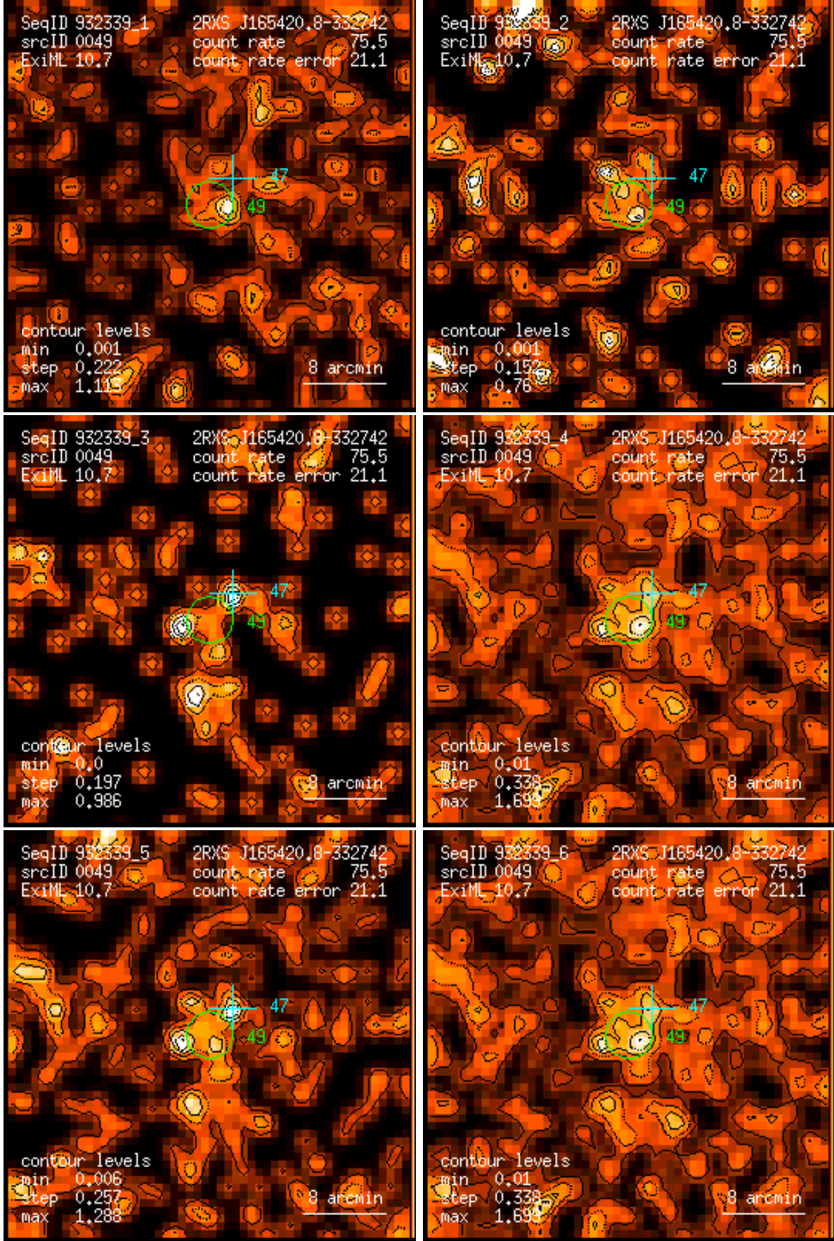
Figure 49: RASS 932339: detection 0049: band rate images, Gaussian filter: (1) PSPC channels 11 – 41, (2) 52 – 90, (3) 91 – 201, (4) 11 – 235, (5) 52 – 201, (6) 11 – 201. Broad band rates in counts/ks. Band rate contour levels in counts/ks/arcmin 2 .
