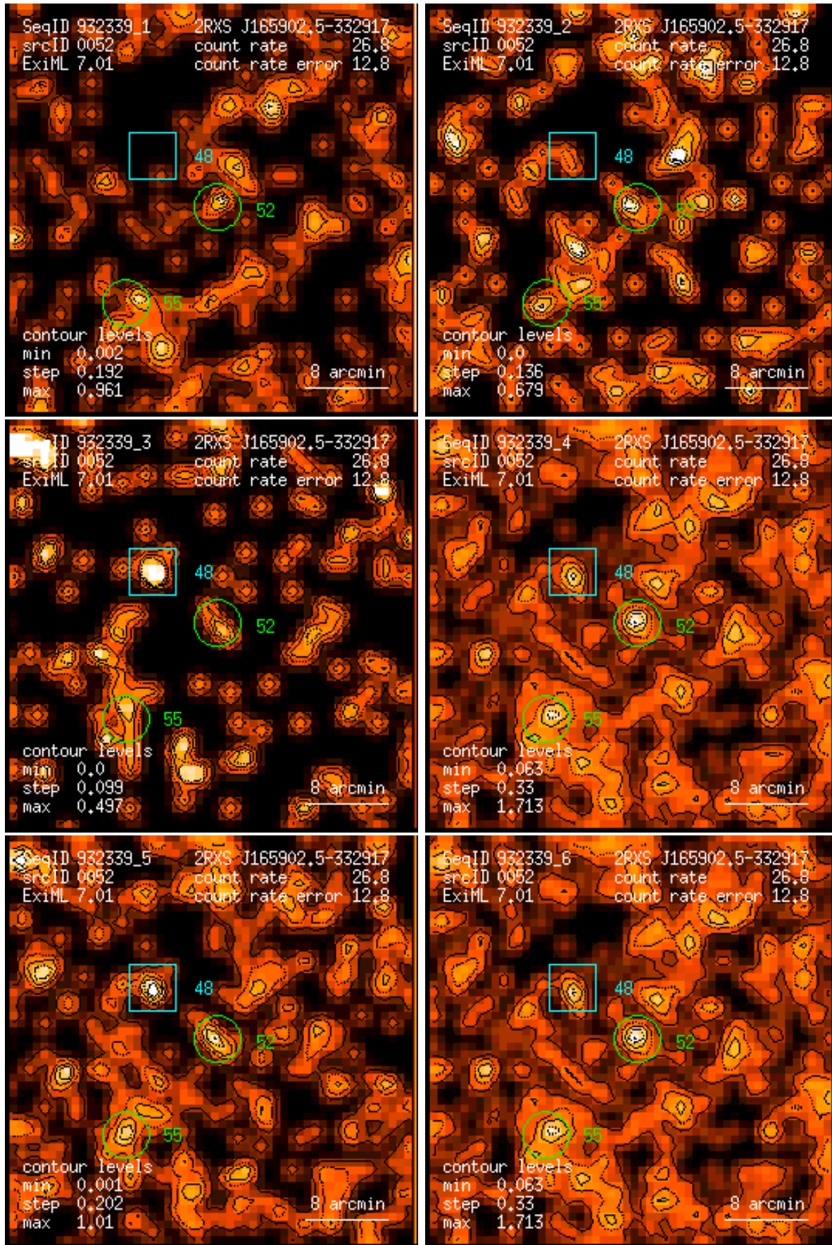
Figure 52: RASS 932339: detection 0052: band rate images, Gaussian filter: (1) PSPC channels 11 – 41, (2) 52 – 90, (3) 91 – 201, (4) 11 – 235, (5) 52 – 201, (6) 11 – 201. Broad band rates in counts/ks. Band rate contour levels in counts/ks/arcmin 2 .
