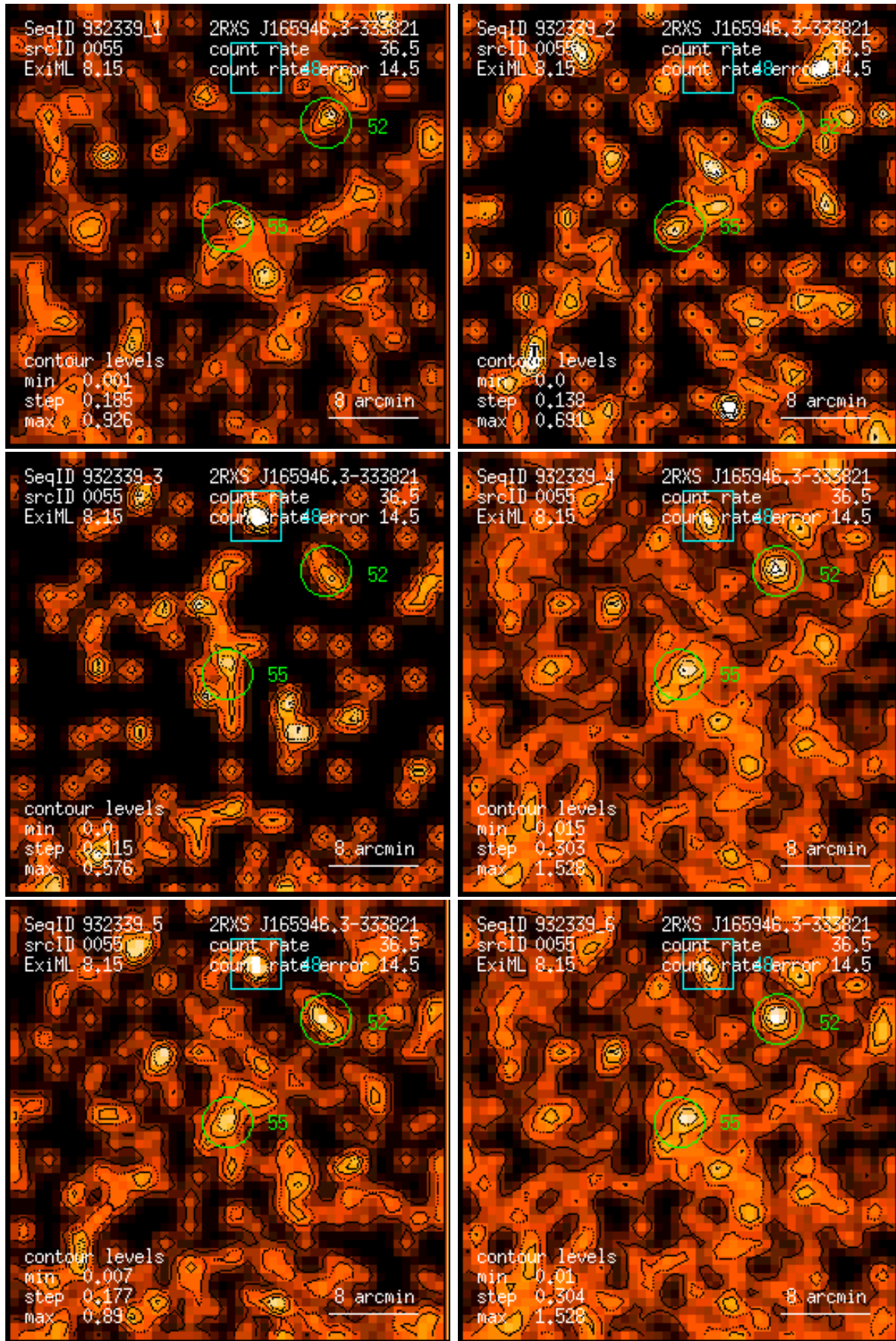
Figure 55: RASS 932339: detection 0055: band rate images, Gaussian filter: (1) PSPC channels 11 – 41, (2) 52 – 90, (3) 91 – 201, (4) 11 – 235, (5) 52 – 201, (6) 11 – 201. Broad band rates in counts/ks. Band rate contour levels in counts/ks/arcmin 2 .
