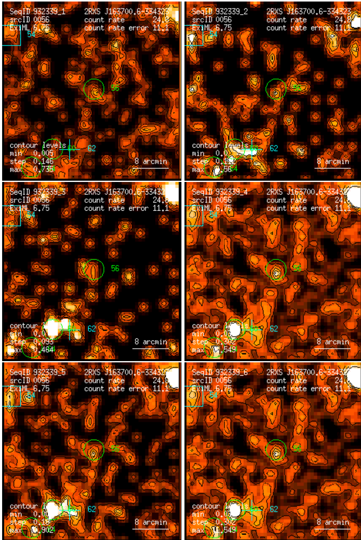
Figure 56: RASS 932339: detection 0056: band rate images, Gaussian filter: (1) PSPC channels 11 – 41, (2) 52 – 90, (3) 91 – 201, (4) 11 – 235, (5) 52 – 201, (6) 11 – 201. Broad band rates in counts/ks. Band rate contour levels in counts/ks/arcmin 2 .
