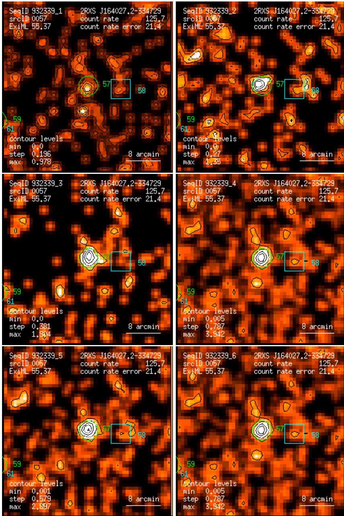
Figure 57: RASS 932339: detection 0057: band rate images, Gaussian filter: (1) PSPC channels 11 – 41, (2) 52 – 90, (3) 91 – 201, (4) 11 – 235, (5) 52 – 201, (6) 11 – 201. Broad band rates in counts/ks. Band rate contour levels in counts/ks/arcmin 2 .
