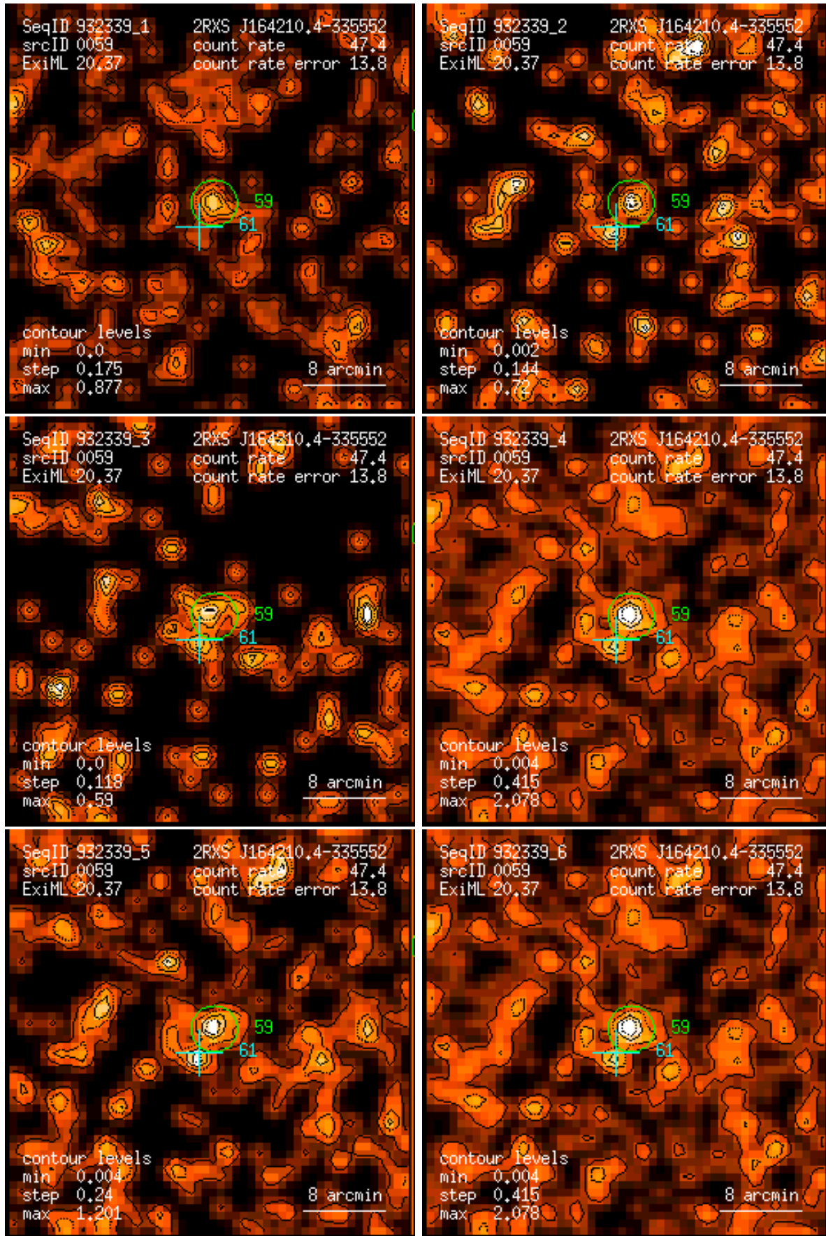
Figure 59: RASS 932339: detection 0059: band rate images, Gaussian filter: (1) PSPC channels 11 – 41, (2) 52 – 90, (3) 91 – 201, (4) 11 – 235, (5) 52 – 201, (6) 11 – 201. Broad band rates in counts/ks. Band rate contour levels in counts/ks/arcmin 2 .
