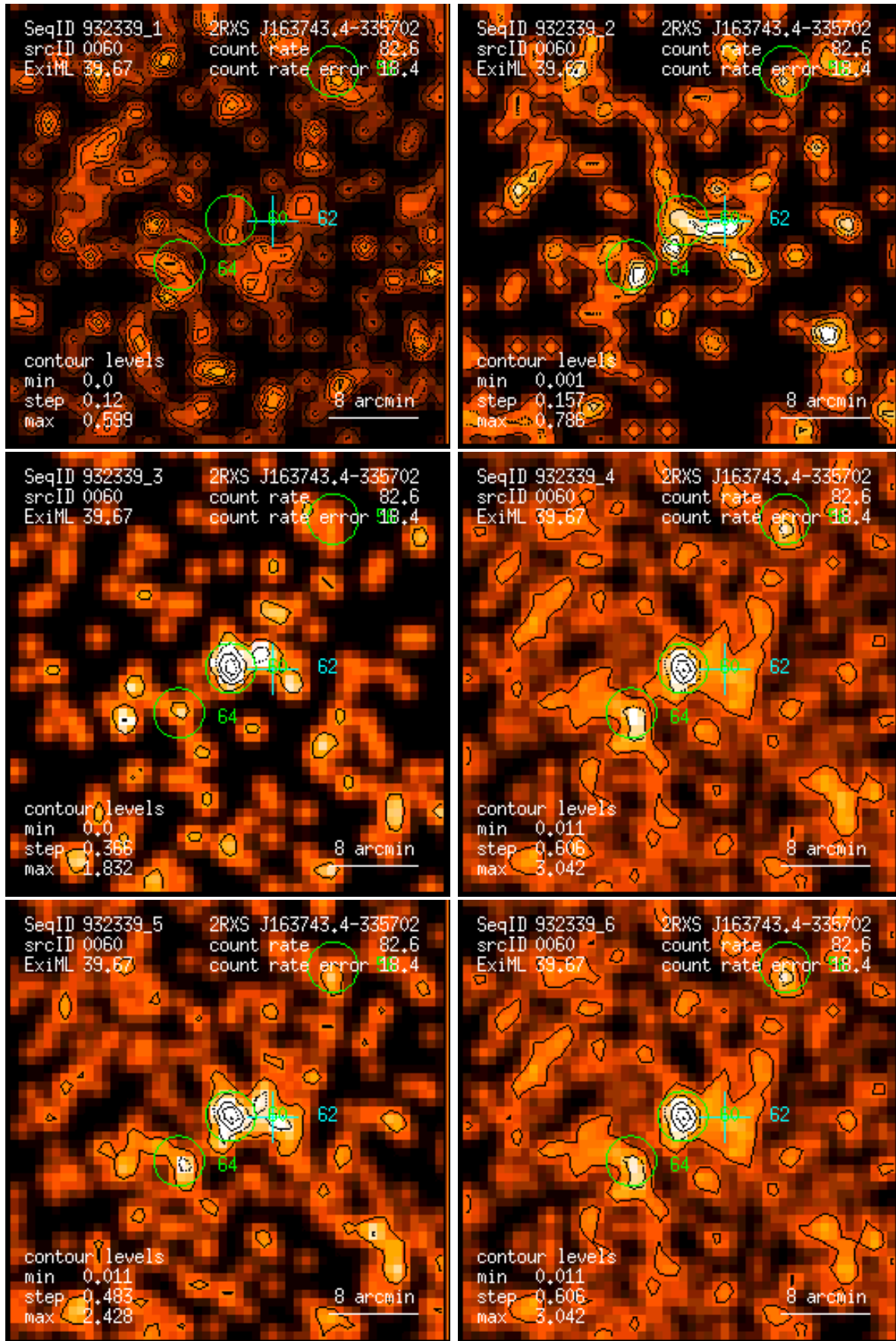
Figure 60: RASS 932339: detection 0060: band rate images, Gaussian filter: (1) PSPC channels 11 – 41, (2) 52 – 90, (3) 91 – 201, (4) 11 – 235, (5) 52 – 201, (6) 11 – 201. Broad band rates in counts/ks. Band rate contour levels in counts/ks/arcmin 2 .
