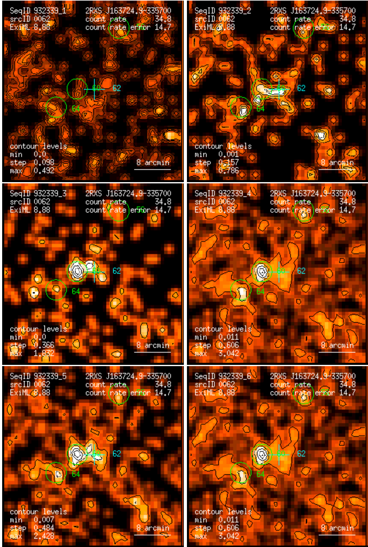
Figure 62: RASS 932339: detection 0062: band rate images, Gaussian filter: (1) PSPC channels 11 – 41, (2) 52 – 90, (3) 91 – 201, (4) 11 – 235, (5) 52 – 201, (6) 11 – 201. Broad band rates in counts/ks. Band rate contour levels in counts/ks/arcmin 2 .
