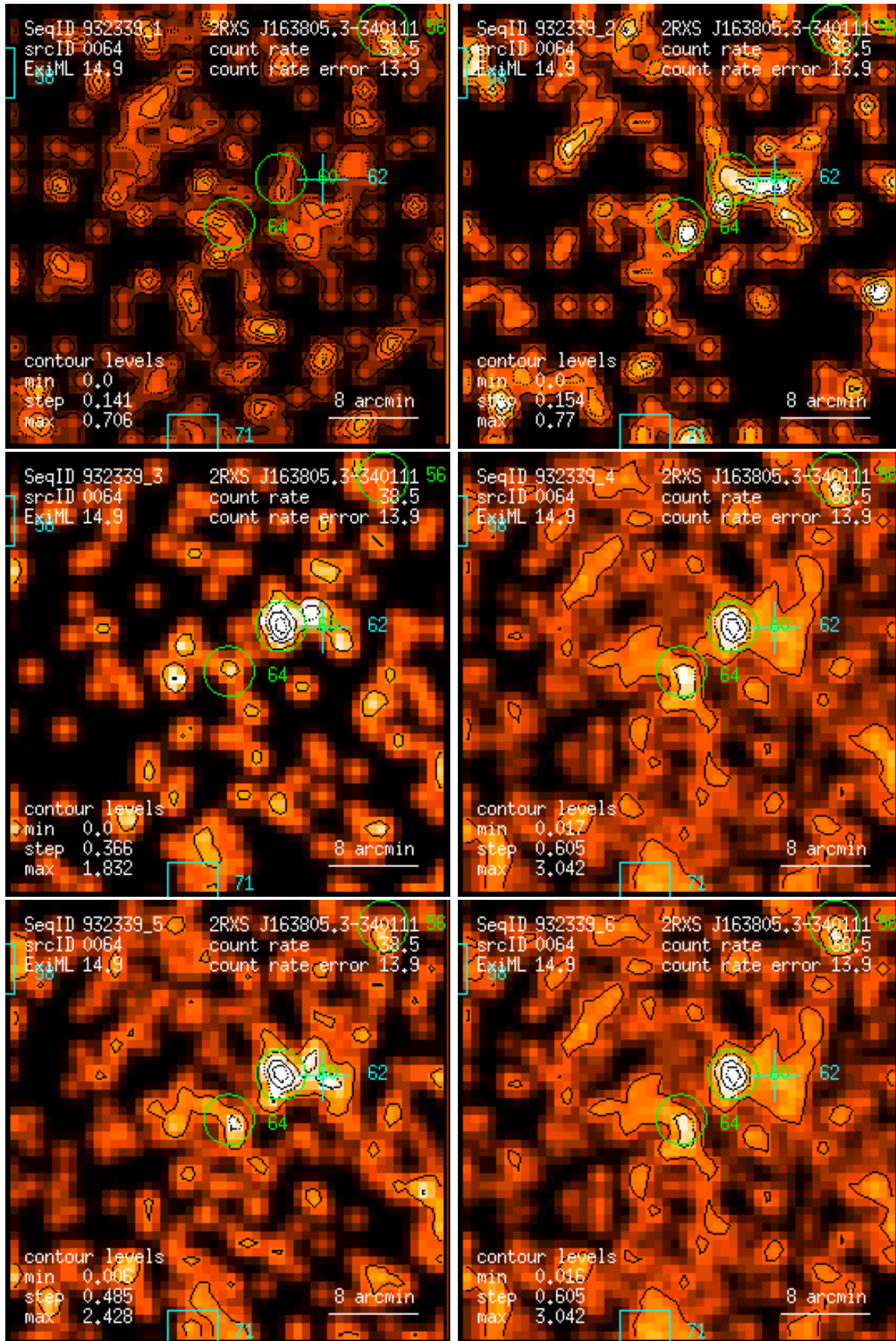
Figure 64: RASS 932339: detection 0064: band rate images, Gaussian filter: (1) PSPC channels 11 – 41, (2) 52 – 90, (3) 91 – 201, (4) 11 – 235, (5) 52 – 201, (6) 11 – 201. Broad band rates in counts/ks. Band rate contour levels in counts/ks/arcmin 2 .
