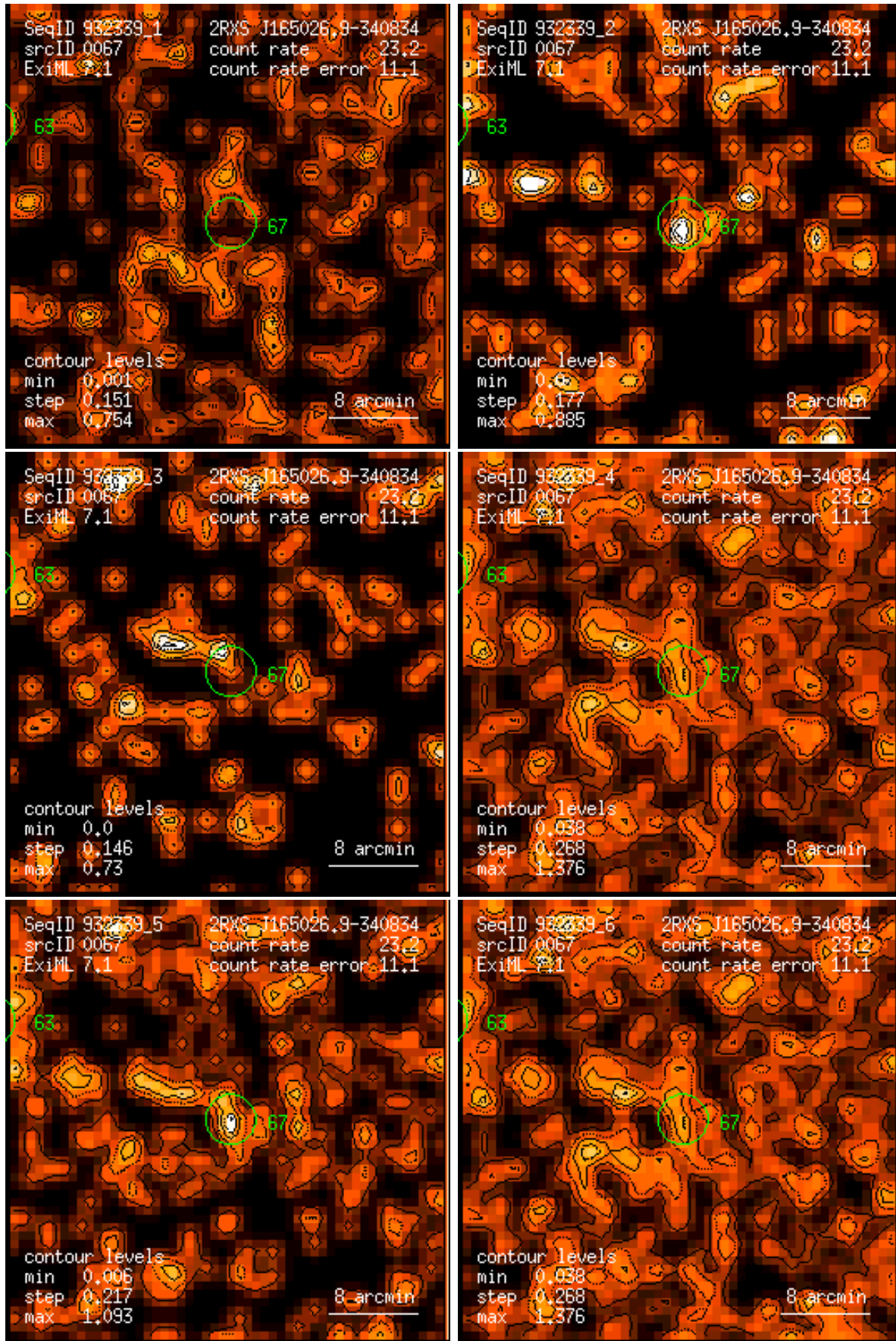
Figure 67: RASS 932339: detection 0067: band rate images, Gaussian filter: (1) PSPC channels 11 – 41, (2) 52 – 90, (3) 91 – 201, (4) 11 – 235, (5) 52 – 201, (6) 11 – 201. Broad band rates in counts/ks. Band rate contour levels in counts/ks/arcmin 2 .
