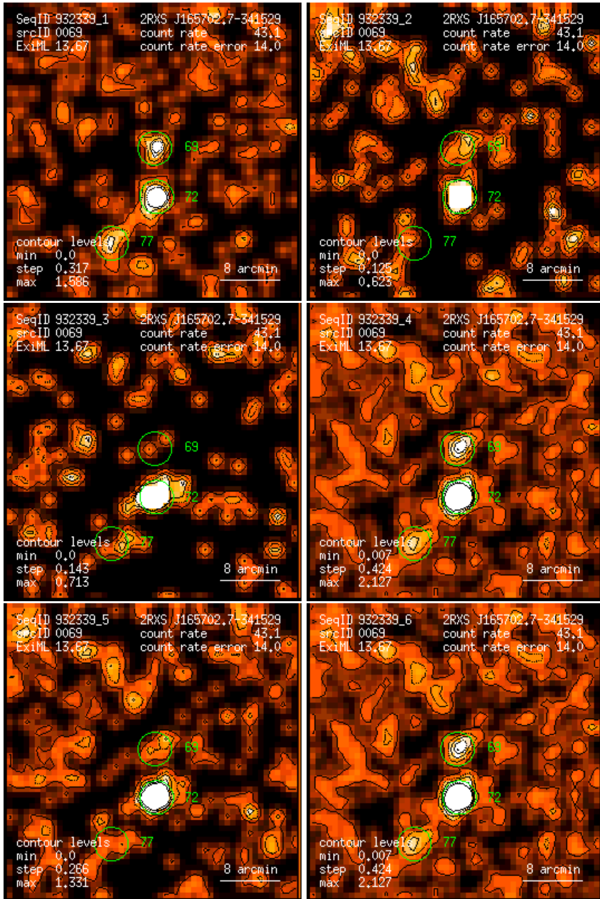
Figure 69: RASS 932339: detection 0069: band rate images, Gaussian filter: (1) PSPC channels 11 – 41, (2) 52 – 90, (3) 91 – 201, (4) 11 – 235, (5) 52 – 201, (6) 11 – 201. Broad band rates in counts/ks. Band rate contour levels in counts/ks/arcmin 2 .
