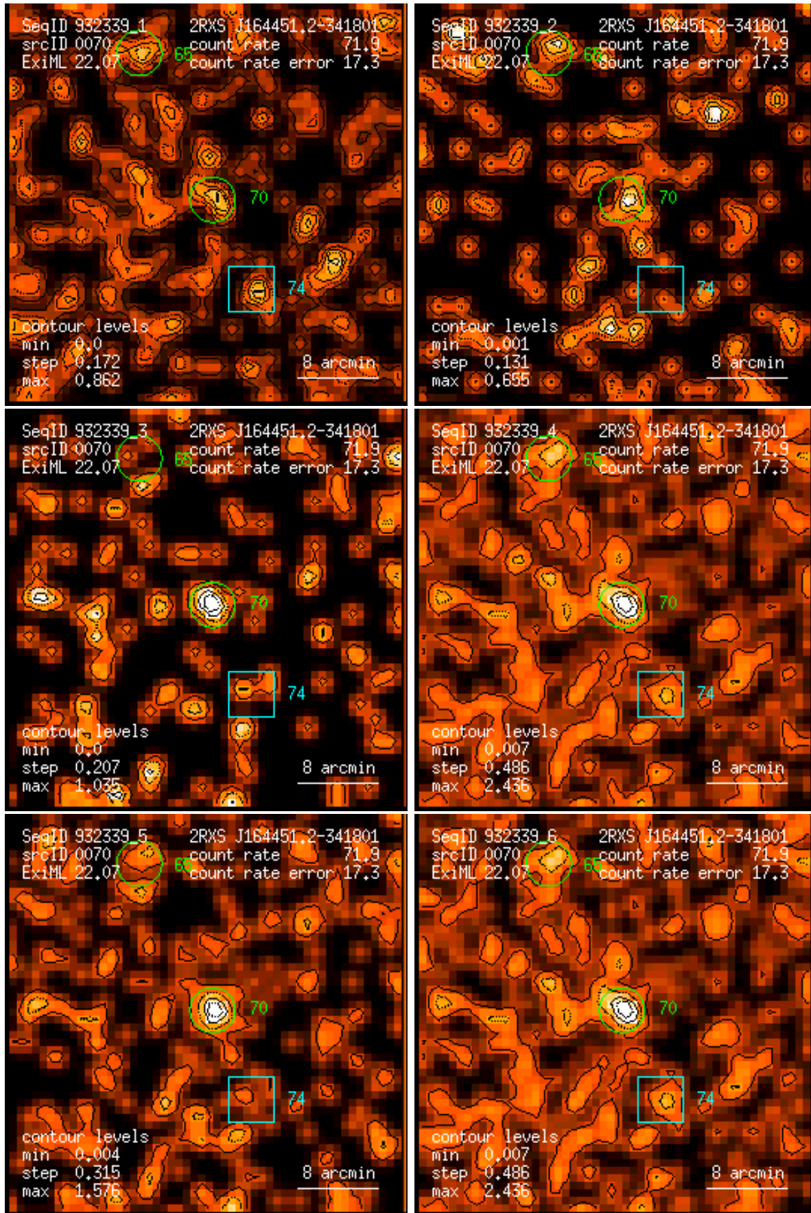
Figure 70: RASS 932339: detection 0070: band rate images, Gaussian filter: (1) PSPC channels 11 – 41, (2) 52 – 90, (3) 91 – 201, (4) 11 – 235, (5) 52 – 201, (6) 11 – 201. Broad band rates in counts/ks. Band rate contour levels in counts/ks/arcmin 2 .
