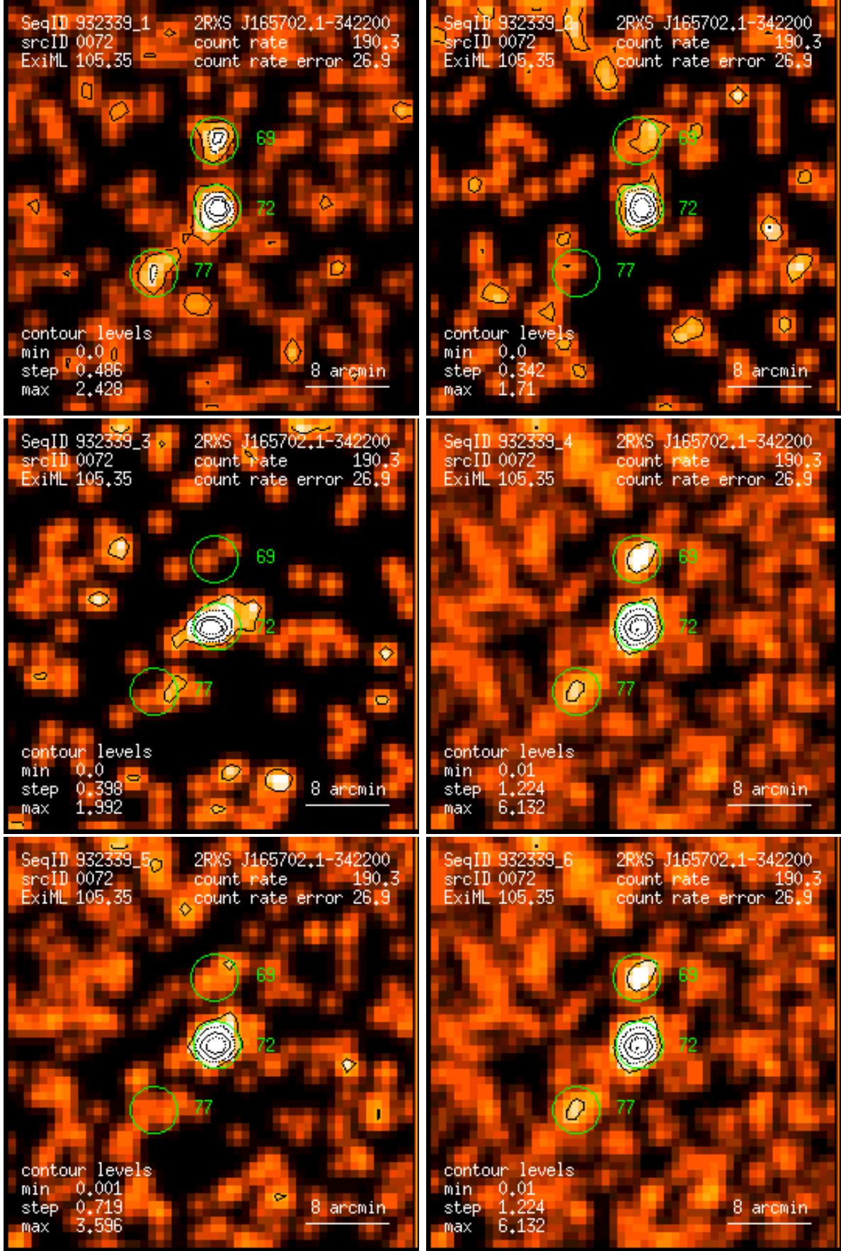
Figure 72: RASS 932339: detection 0072: band rate images, Gaussian filter: (1) PSPC channels 11 – 41, (2) 52 – 90, (3) 91 – 201, (4) 11 – 235, (5) 52 – 201, (6) 11 – 201. Broad band rates in counts/ks. Band rate contour levels in counts/ks/arcmin 2 .
