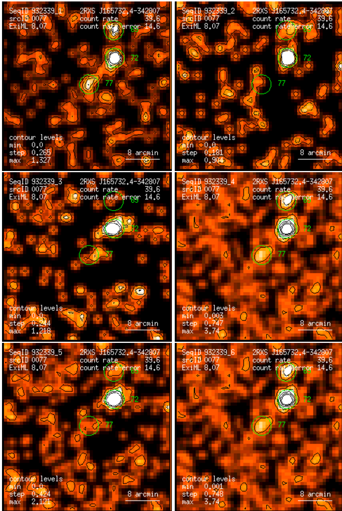
Figure 77: RASS 932339: detection 0077: band rate images, Gaussian filter: (1) PSPC channels 11 – 41, (2) 52 – 90, (3) 91 – 201, (4) 11 – 235, (5) 52 – 201, (6) 11 – 201. Broad band rates in counts/ks. Band rate contour levels in counts/ks/arcmin 2 .
