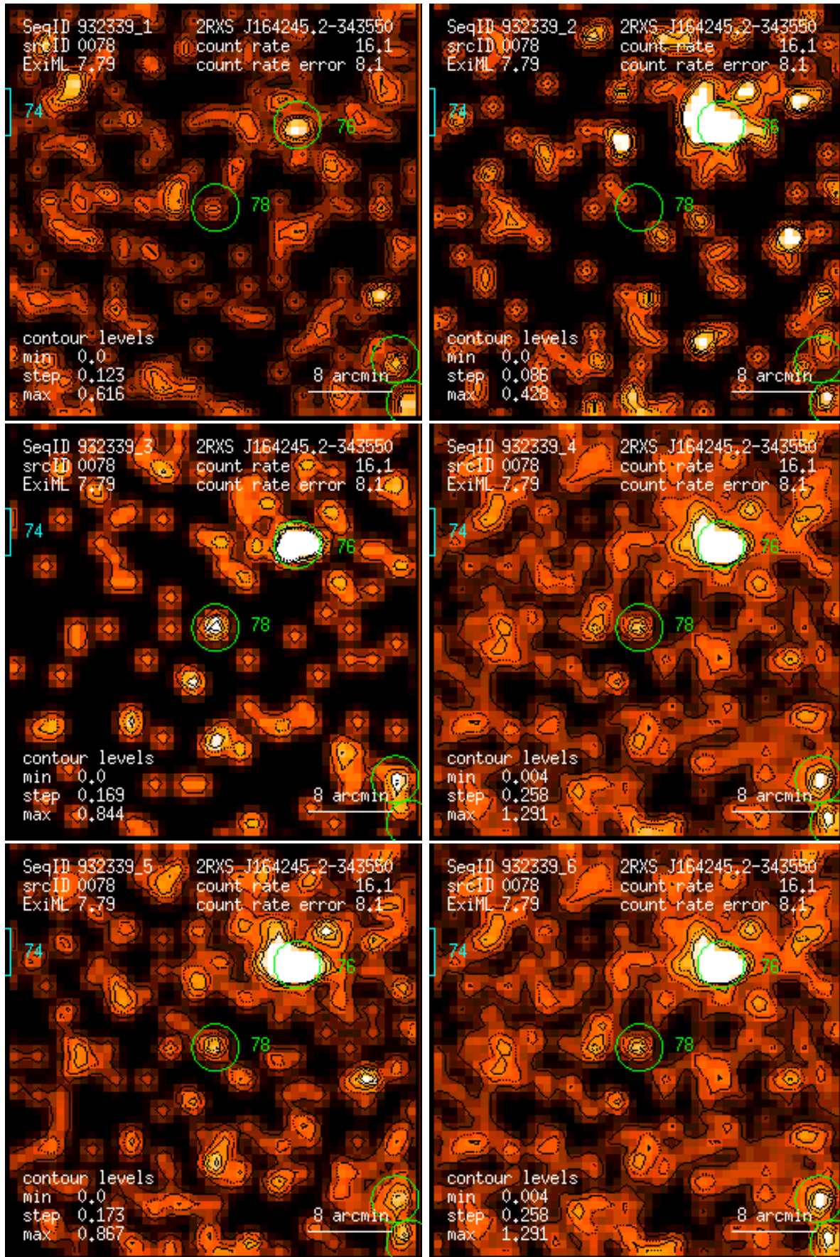
Figure 78: RASS 932339: detection 0078: band rate images, Gaussian filter: (1) PSPC channels 11 – 41, (2) 52 – 90, (3) 91 – 201, (4) 11 – 235, (5) 52 – 201, (6) 11 – 201. Broad band rates in counts/ks. Band rate contour levels in counts/ks/arcmin 2 .
