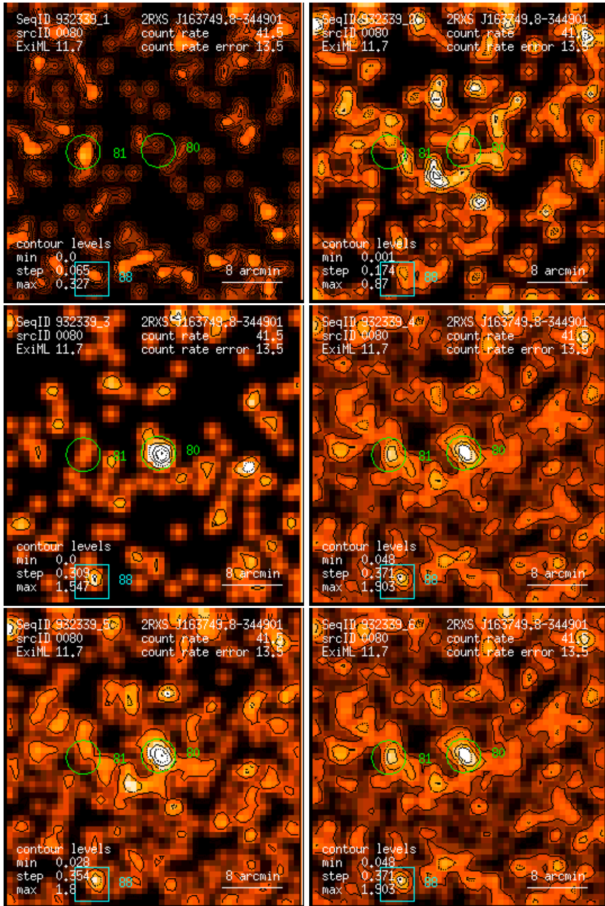
Figure 80: RASS 932339: detection 0080: band rate images, Gaussian filter: (1) PSPC channels 11 – 41, (2) 52 – 90, (3) 91 – 201, (4) 11 – 235, (5) 52 – 201, (6) 11 – 201. Broad band rates in counts/ks. Band rate contour levels in counts/ks/arcmin 2 .
