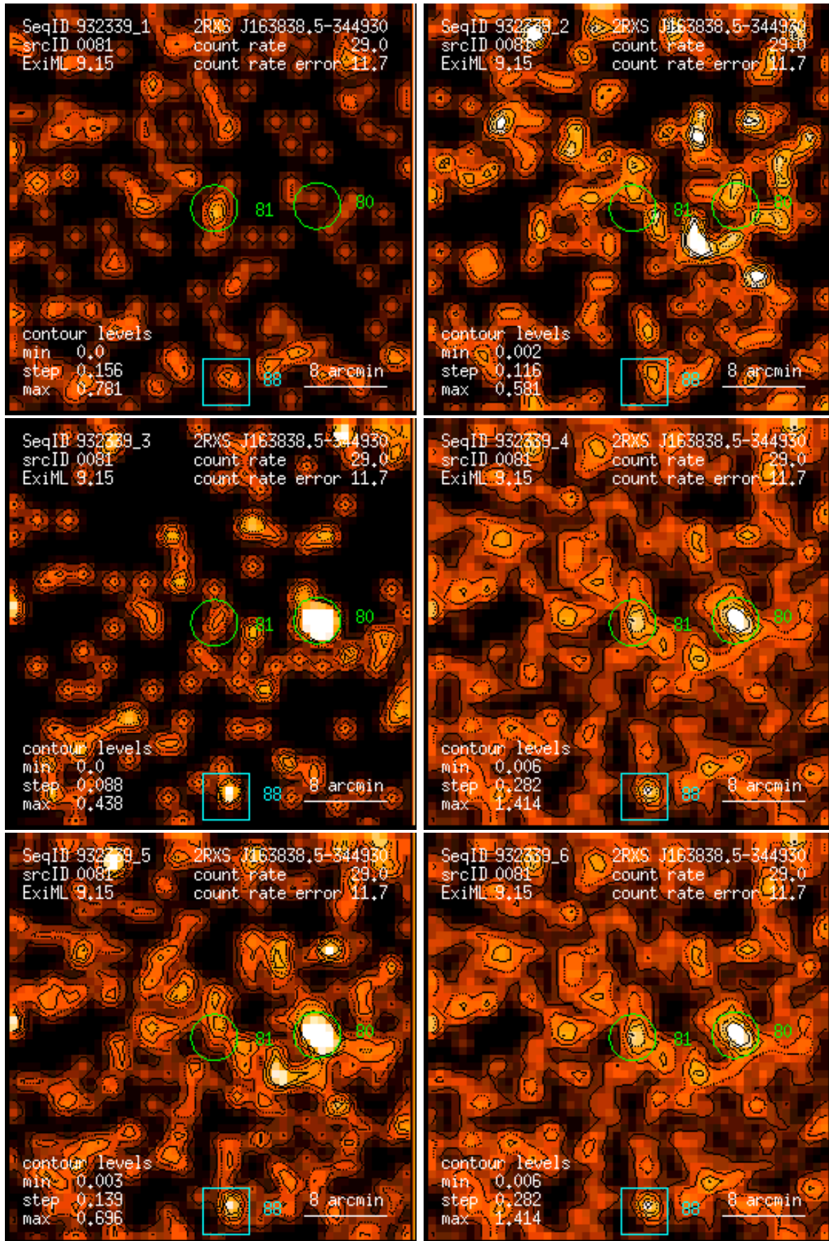
Figure 81: RASS 932339: detection 0081: band rate images, Gaussian filter: (1) PSPC channels 11 – 41, (2) 52 – 90, (3) 91 – 201, (4) 11 – 235, (5) 52 – 201, (6) 11 – 201. Broad band rates in counts/ks. Band rate contour levels in counts/ks/arcmin 2 .
