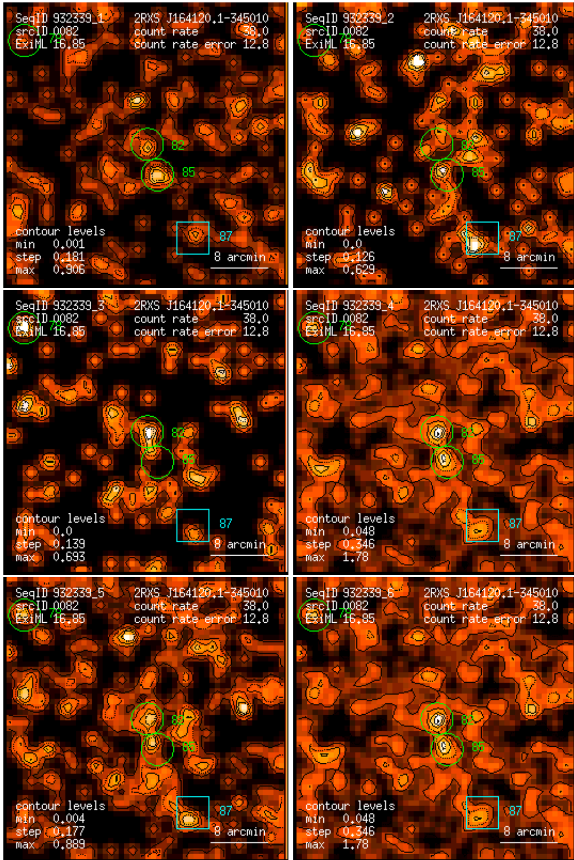
Figure 82: RASS 932339: detection 0082: band rate images, Gaussian filter: (1) PSPC channels 11 – 41, (2) 52 – 90, (3) 91 – 201, (4) 11 – 235, (5) 52 – 201, (6) 11 – 201. Broad band rates in counts/ks. Band rate contour levels in counts/ks/arcmin 2 .
