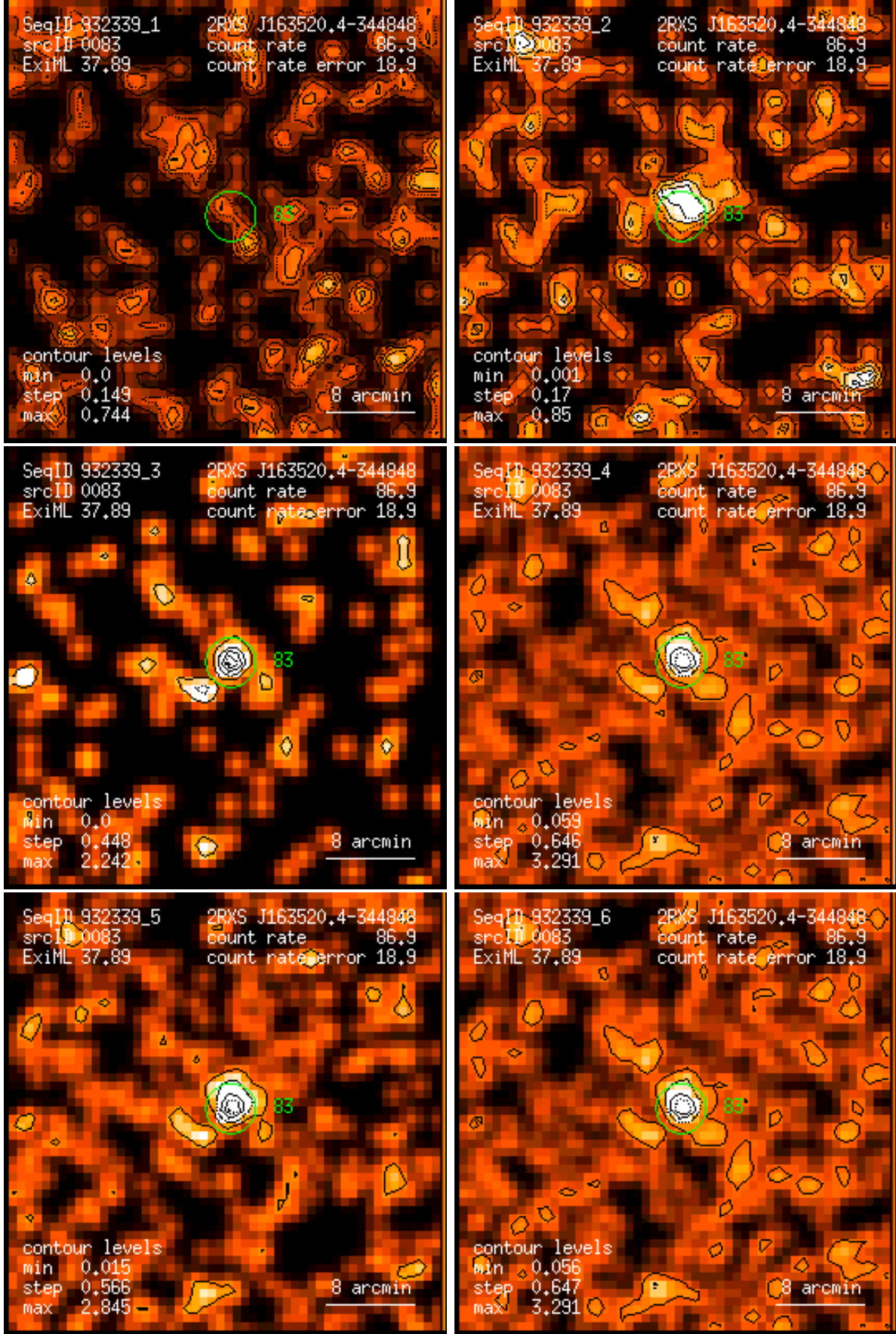
Figure 83: RASS 932339: detection 0083: band rate images, Gaussian filter: (1) PSPC channels 11 – 41, (2) 52 – 90, (3) 91 – 201, (4) 11 – 235, (5) 52 – 201, (6) 11 – 201. Broad band rates in counts/ks. Band rate contour levels in counts/ks/arcmin 2 .
