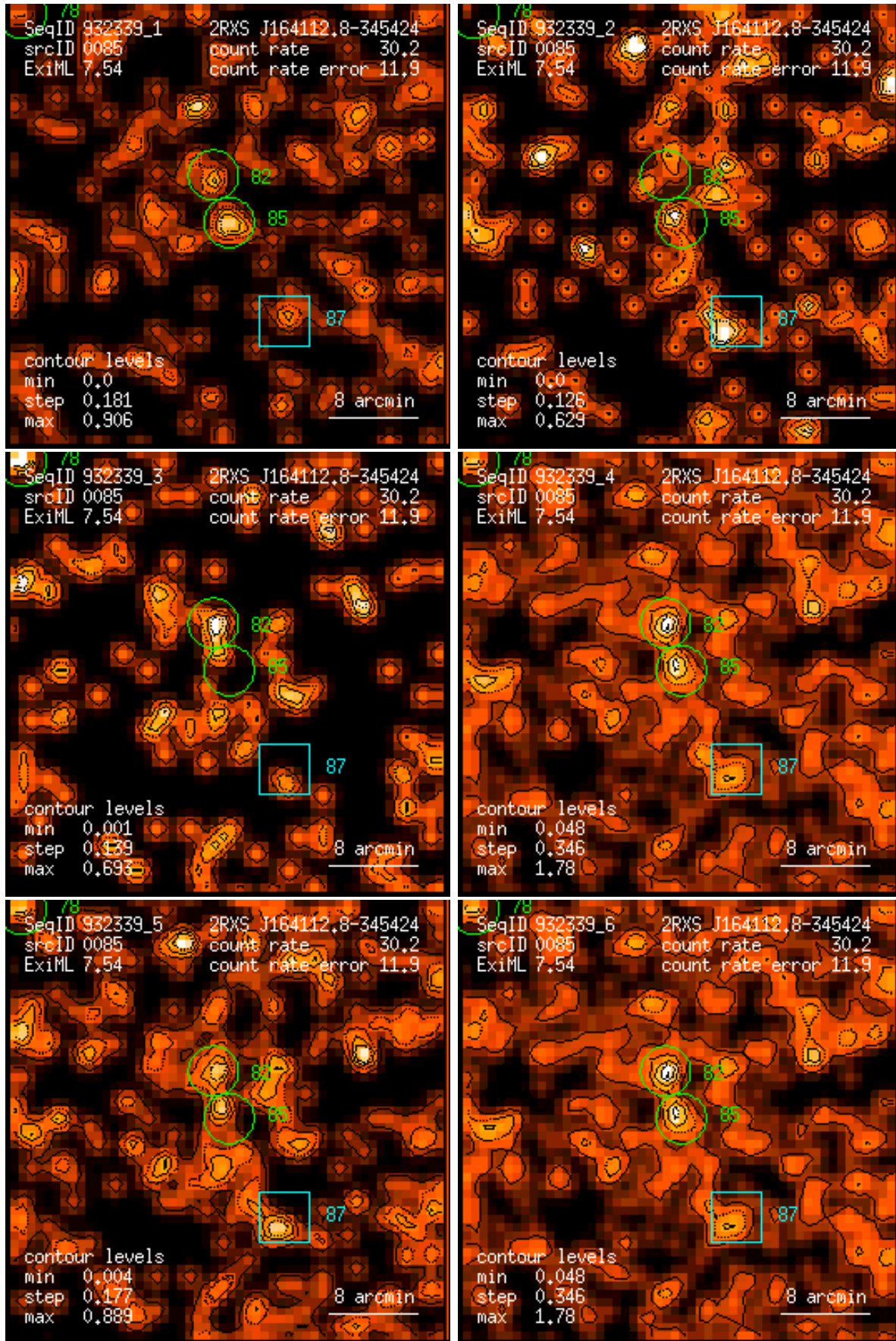
Figure 85: RASS 932339: detection 0085: band rate images, Gaussian filter: (1) PSPC channels 11 – 41, (2) 52 – 90, (3) 91 – 201, (4) 11 – 235, (5) 52 – 201, (6) 11 – 201. Broad band rates in counts/ks. Band rate contour levels in counts/ks/arcmin 2 .
