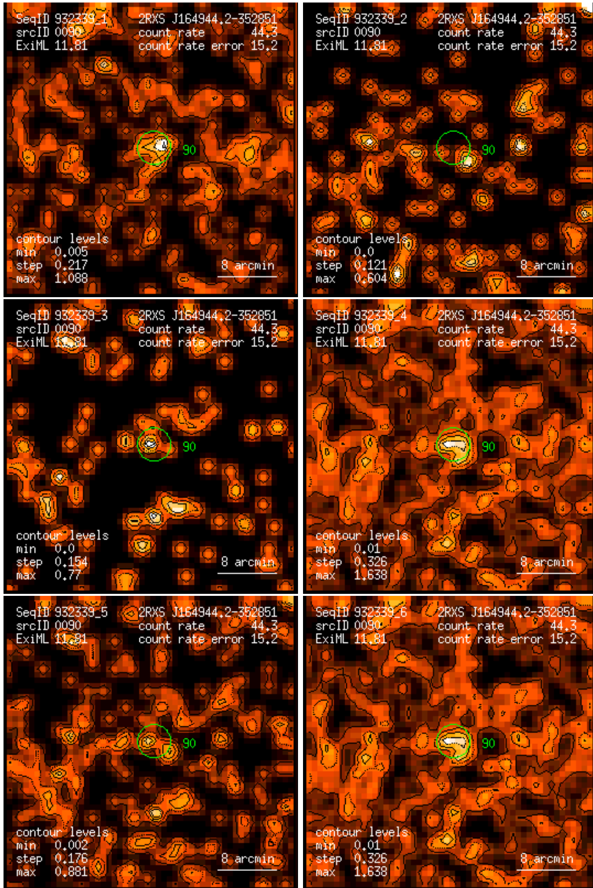
Figure 90: RASS 932339: detection 0090: band rate images, Gaussian filter: (1) PSPC channels 11 – 41, (2) 52 – 90, (3) 91 – 201, (4) 11 – 235, (5) 52 – 201, (6) 11 – 201. Broad band rates in counts/ks. Band rate contour levels in counts/ks/arcmin 2 .
