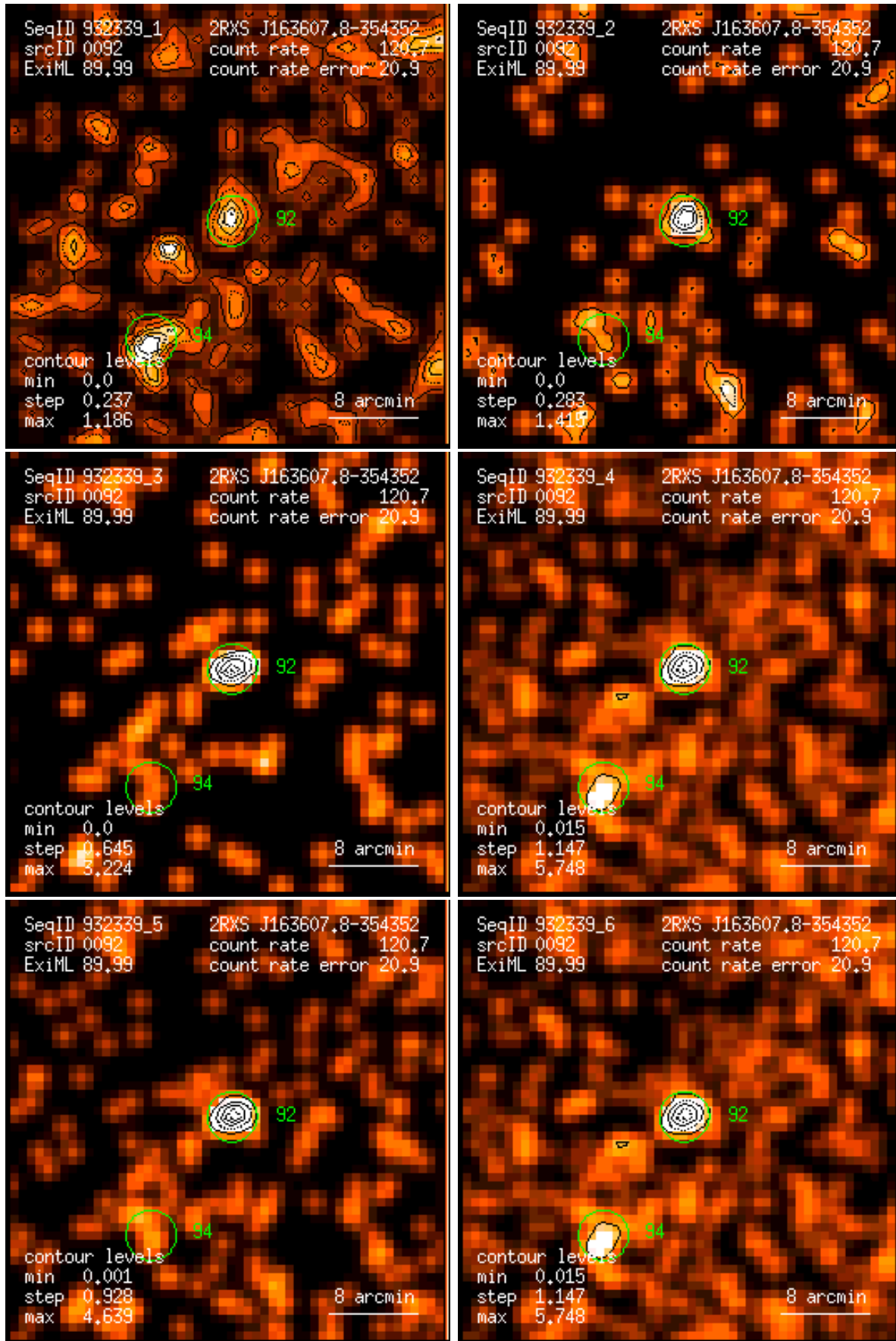
Figure 92: RASS 932339: detection 0092: band rate images, Gaussian filter: (1) PSPC channels 11 – 41, (2) 52 – 90, (3) 91 – 201, (4) 11 – 235, (5) 52 – 201, (6) 11 – 201. Broad band rates in counts/ks. Band rate contour levels in counts/ks/arcmin 2 .
