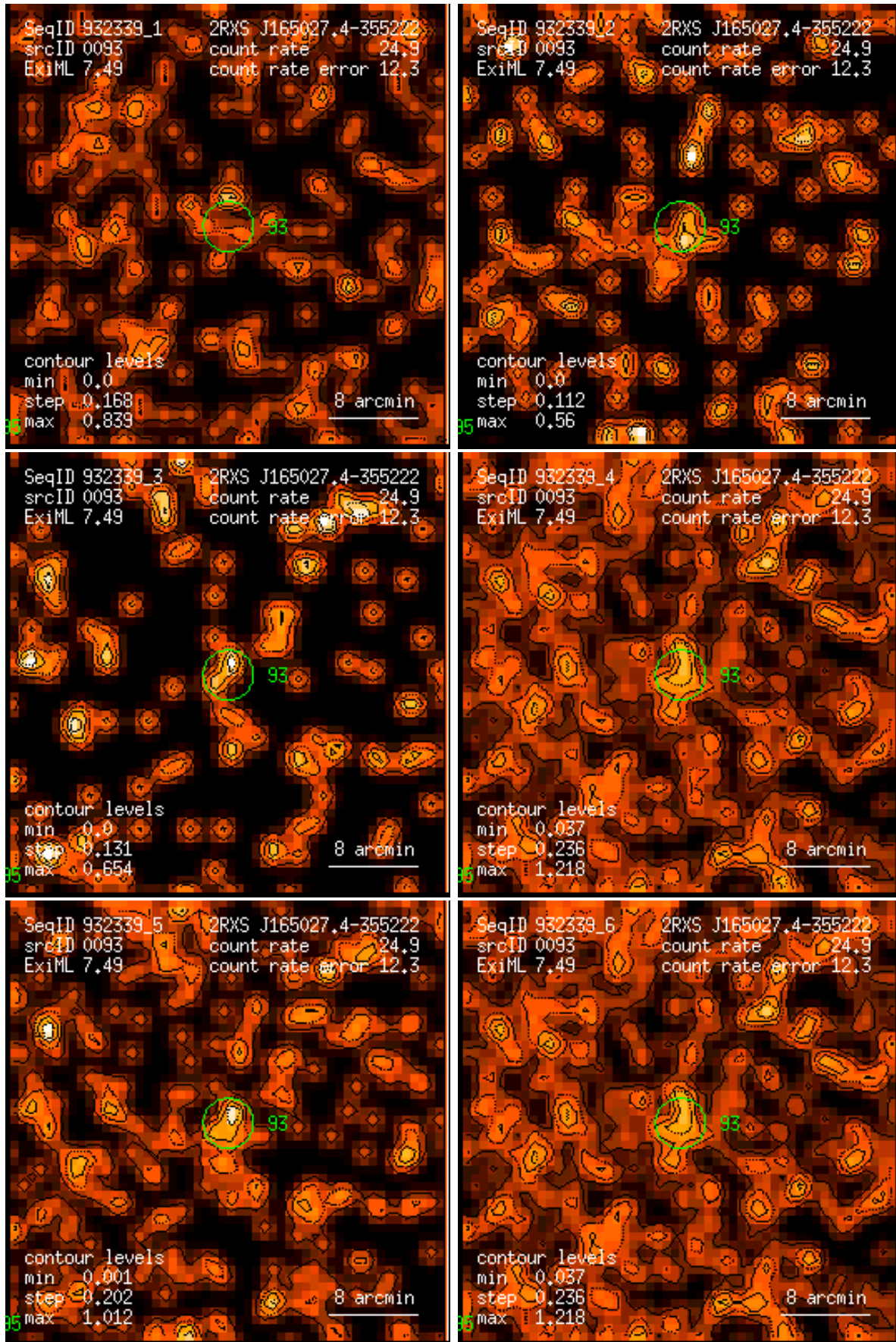
Figure 93: RASS 932339: detection 0093: band rate images, Gaussian filter: (1) PSPC channels 11 – 41, (2) 52 – 90, (3) 91 – 201, (4) 11 – 235, (5) 52 – 201, (6) 11 – 201. Broad band rates in counts/ks. Band rate contour levels in counts/ks/arcmin 2 .
