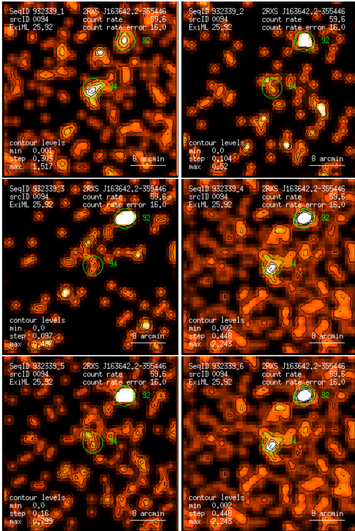
Figure 94: RASS 932339: detection 0094: band rate images, Gaussian filter: (1) PSPC channels 11 – 41, (2) 52 – 90, (3) 91 – 201, (4) 11 – 235, (5) 52 – 201, (6) 11 – 201. Broad band rates in counts/ks. Band rate contour levels in counts/ks/arcmin 2 .
