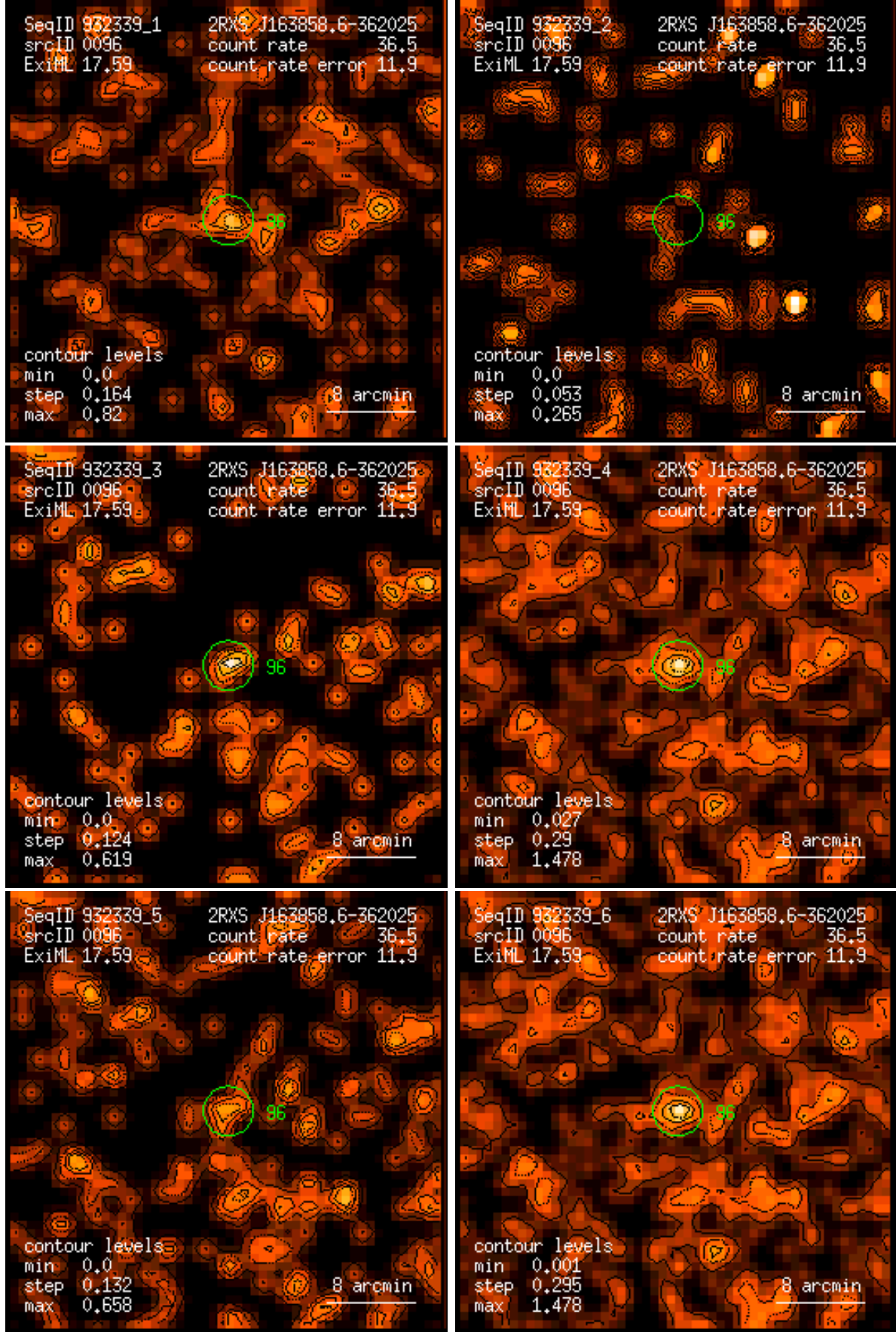
Figure 96: RASS 932339: detection 0096: band rate images, Gaussian filter: (1) PSPC channels 11 – 41, (2) 52 – 90, (3) 91 – 201, (4) 11 – 235, (5) 52 – 201, (6) 11 – 201. Broad band rates in counts/ks. Band rate contour levels in counts/ks/arcmin 2 .
