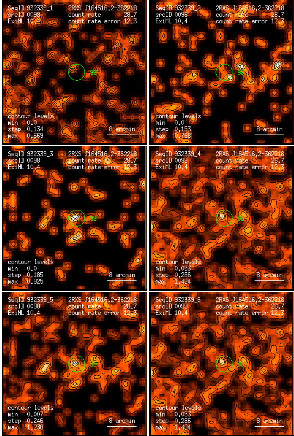
Figure 98: RASS 932339: detection 0098: band rate images, Gaussian filter: (1) PSPC channels 11 – 41, (2) 52 – 90, (3) 91 – 201, (4) 11 – 235, (5) 52 – 201, (6) 11 – 201. Broad band rates in counts/ks. Band rate contour levels in counts/ks/arcmin 2 .
