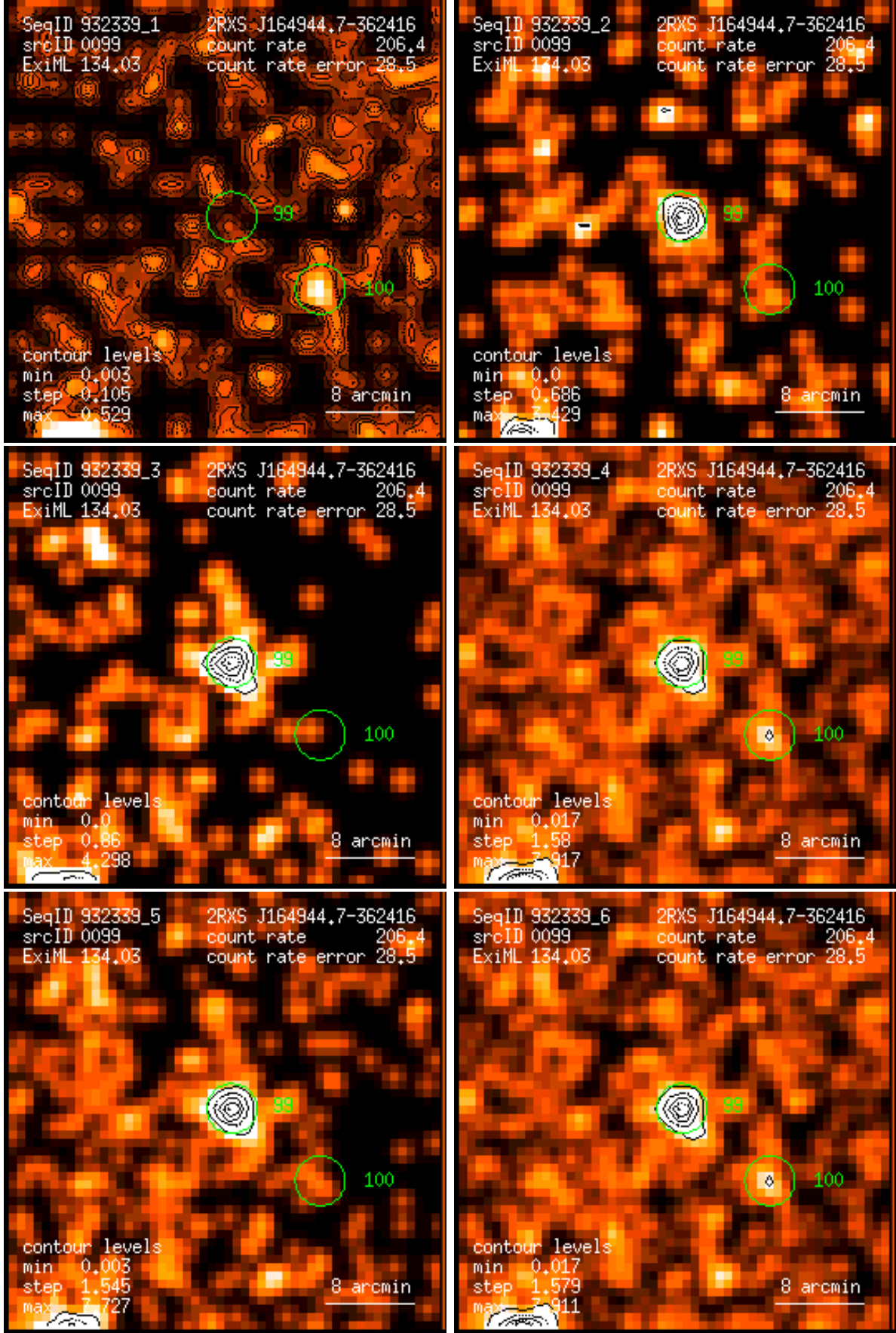
Figure 99: RASS 932339: detection 0099: band rate images, Gaussian filter: (1) PSPC channels 11 – 41, (2) 52 – 90, (3) 91 – 201, (4) 11 – 235, (5) 52 – 201, (6) 11 – 201. Broad band rates in counts/ks. Band rate contour levels in counts/ks/arcmin 2 .
