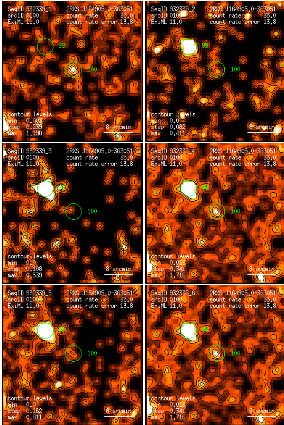
Figure 100: RASS 932339: detection 0100: band rate images, Gaussian filter: (1) PSPC channels 11 – 41, (2) 52 – 90, (3) 91 – 201, (4) 11 – 235, (5) 52 – 201, (6) 11 – 201. Broad band rates in counts/ks. Band rate contour levels in counts/ks/arcmin 2 .
