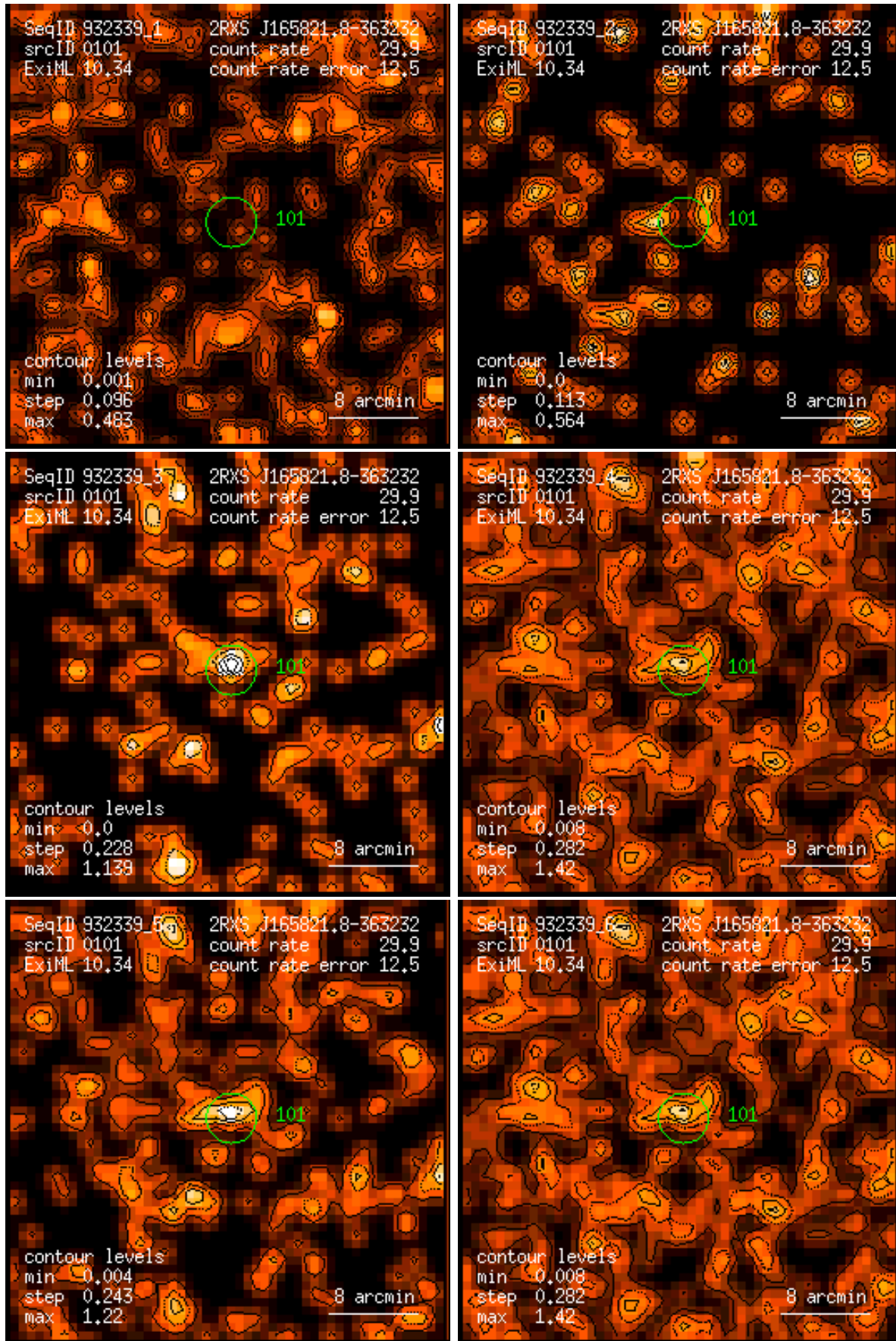
Figure 101: RASS 932339: detection 0101: band rate images, Gaussian filter: (1) PSPC channels 11 – 41, (2) 52 – 90, (3) 91 – 201, (4) 11 – 235, (5) 52 – 201, (6) 11 – 201. Broad band rates in counts/ks. Band rate contour levels in counts/ks/arcmin 2 .
