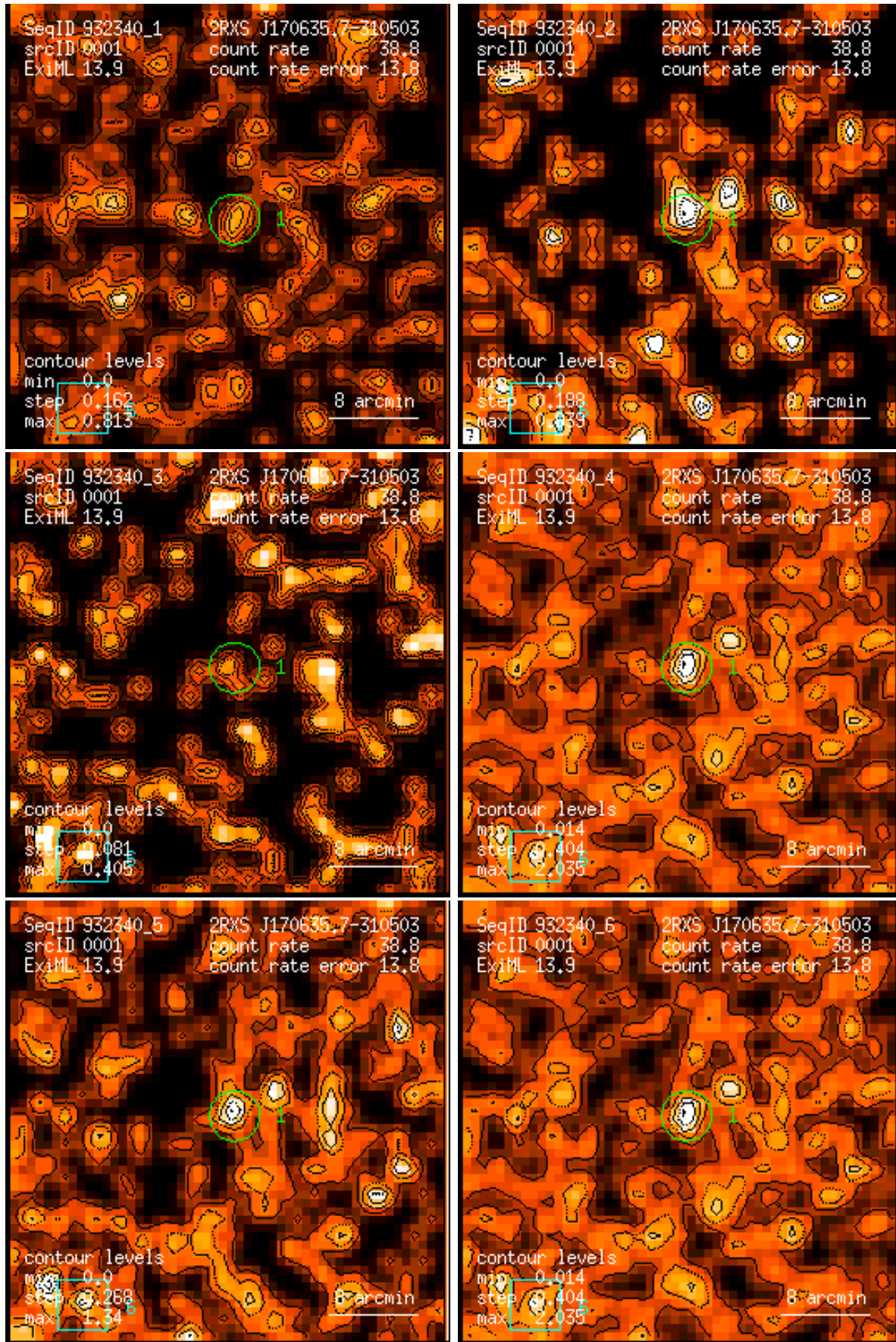
Figure 1: RASS 932340: detection 0001: band rate images, Gaussian filter: (1) PSPC channels 11 – 41, (2) 52 – 90, (3) 91 – 201, (4) 11 – 235, (5) 52 – 201, (6) 11 – 201. Broad band rates in counts/ks. Band rate contour levels in counts/ks/arcmin 2 .
