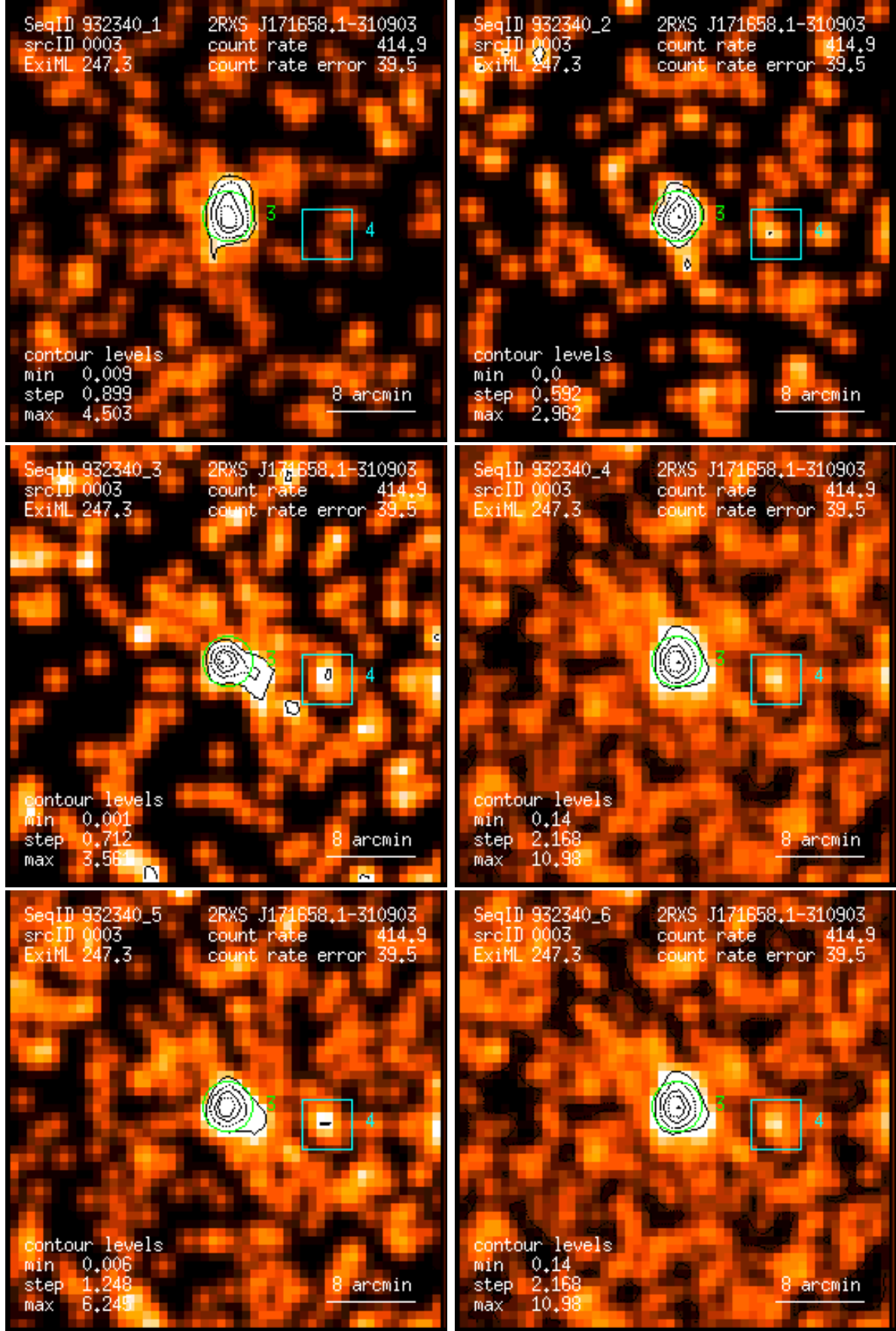
Figure 3: RASS 932340: detection 0003: band rate images, Gaussian filter: (1) PSPC channels 11 – 41, (2) 52 – 90, (3) 91 – 201, (4) 11 – 235, (5) 52 – 201, (6) 11 – 201. Broad band rates in counts/ks. Band rate contour levels in counts/ks/arcmin 2 .
