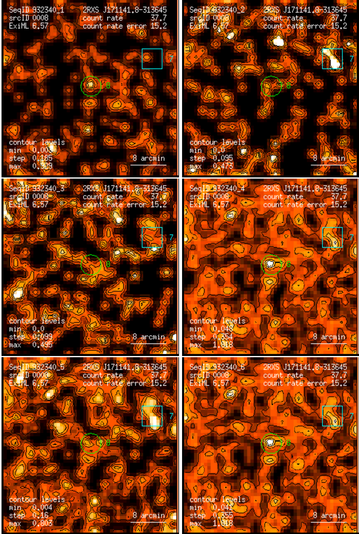
Figure 8: RASS 932340: detection 0008: band rate images, Gaussian filter: (1) PSPC channels 11 – 41, (2) 52 – 90, (3) 91 – 201, (4) 11 – 235, (5) 52 – 201, (6) 11 – 201. Broad band rates in counts/ks. Band rate contour levels in counts/ks/arcmin 2 .
