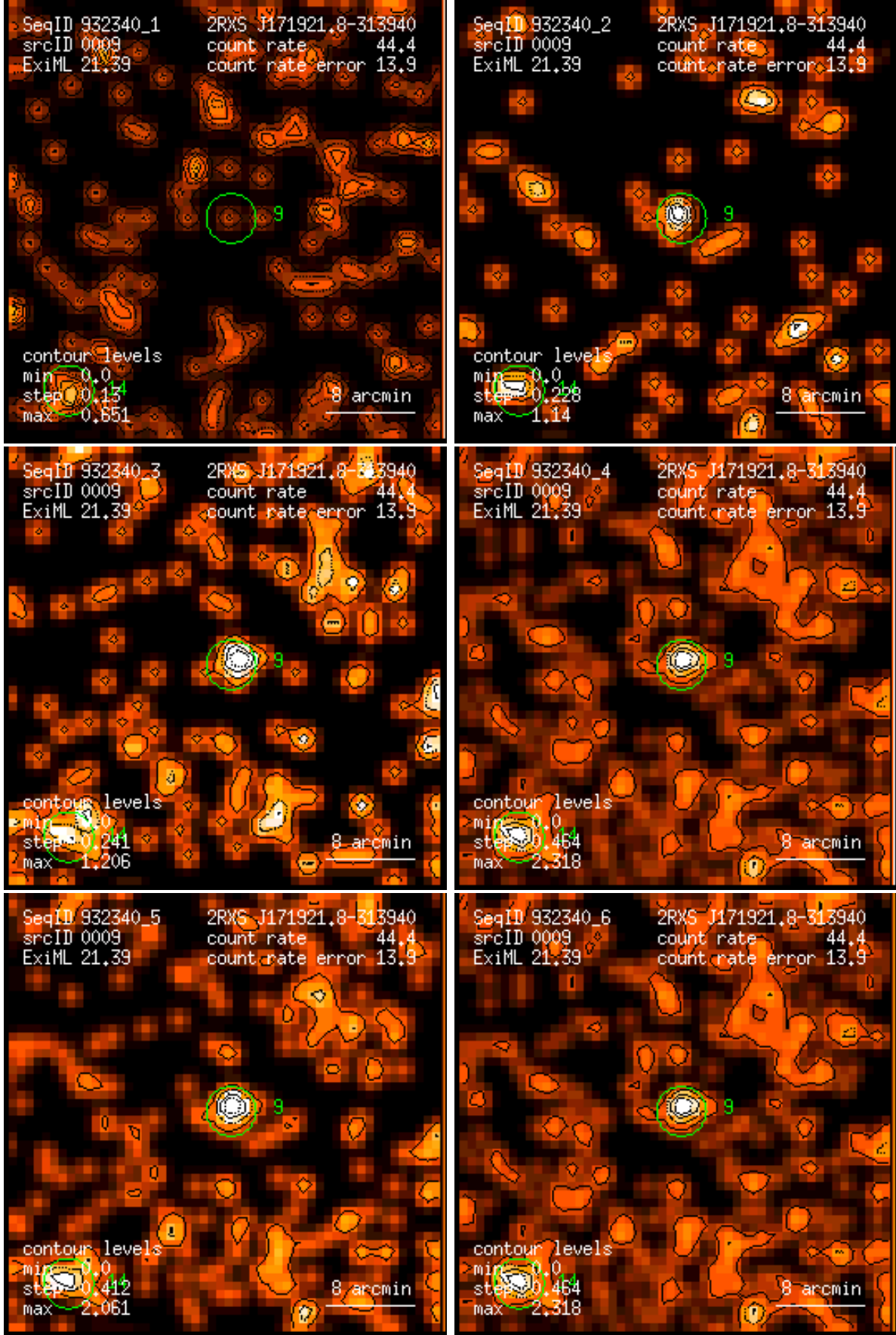
Figure 9: RASS 932340: detection 0009: band rate images, Gaussian filter: (1) PSPC channels 11 – 41, (2) 52 – 90, (3) 91 – 201, (4) 11 – 235, (5) 52 – 201, (6) 11 – 201. Broad band rates in counts/ks. Band rate contour levels in counts/ks/arcmin 2 .
